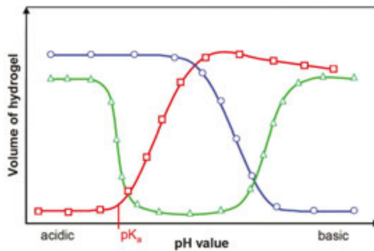
Figure 11. Phase transition behavior of polyelectrolyte hydrogels. Acidic hydrogels (□) are ionized by deprotonation in basic solutions. Basic hydrogels (○) swell in acidic solutions due to the ionization of their basic groups by protonation. Amphiphilic hydrogels (Δ) contain both acidic and basic groups, therefore they show two-phase transitions.
