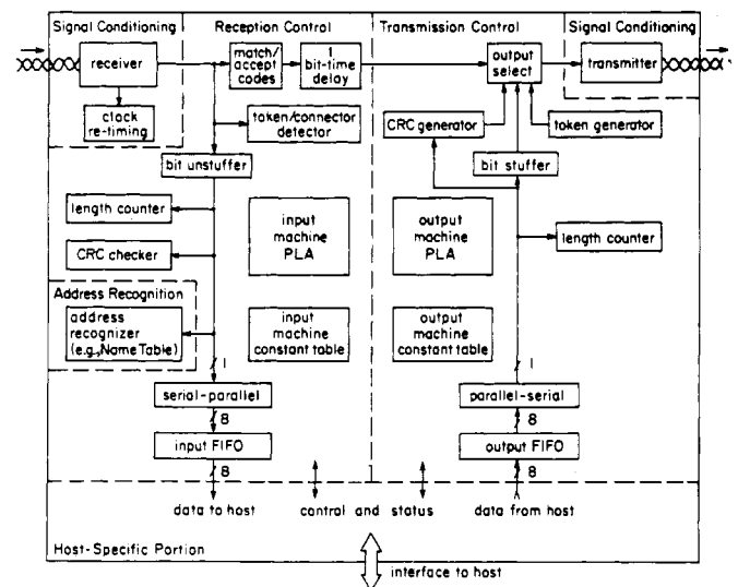
Fig. 6. Block diagram of the Local Network Interface (LNI). The five major components described in the text are separated by dashed lines; the Signal Conditioning Section appears in two parts, at the upper left and upper right. The arrows depict data flow; control, vested in the Programmed Logic Arrays (PLA's) of the input and output machines, is not indicated.
