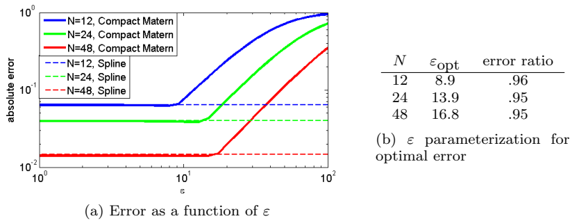
Fig. 7: Error results for iterated Brownian bridge interpolation on the function G_1 from (6.1). The effect of \varepsilon is studied for various N values, and each time an optimal \varepsilon , denoted \varepsilon_{\text{opt}} , produces a smaller error than the spline which occurs in the \varepsilon \rightarrow 0 limit. In the table on the right, the \varepsilon_{\text{opt}} value and the ratio of the optimal error to the spline error is displayed. The N input points were evenly spaced in (0, 1) as were the 400 points at which the error was computed. The spline results were computed with a piecewise linear spline.
