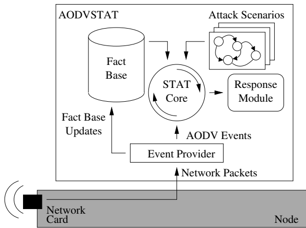
Figure 3. AODVSTAT Sensor Architecture.
