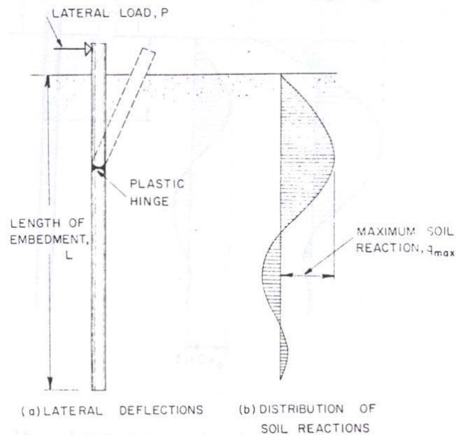
Fig. (2-14) Failure Mode of a Long, Free-Headed Pile (Broms, 1964a)
