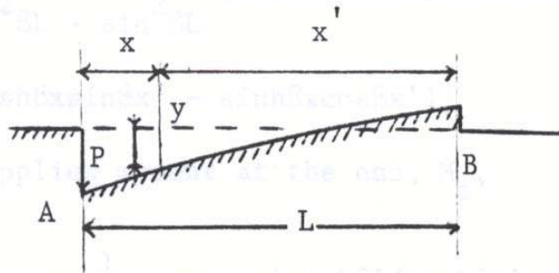
Fig. (1-3) Beam with Concentrated Force at End (Hetenyi, 1942)
