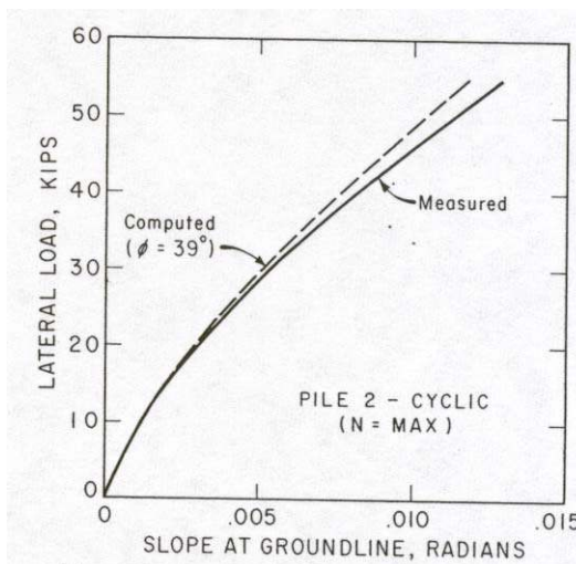
Fig. (3-19) Comparison between Measured Results of Mustang Island Tests and Results Computed with Proposed Criteria; Pile 2 (N = max) Slope at Ground Line (Reese, 1974)
