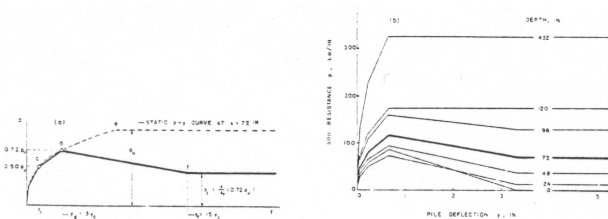
Fig. (3-26) Predicted Cyclic p - y Curves for Sabine Clay and 12.75-inch Dia. Test Pile, based on Static p - y Curves of (a) Typical example, (b) Complete family of Curves (Matlock, 1970)
