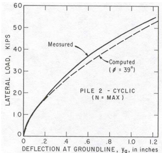
Fig. (3-18) Comparison between Measured Results of Mustang Island Tests and Results Computed with Proposed Criteria; Pile 2 (N = max) Deflection at Ground Line (Reese, 1974)
