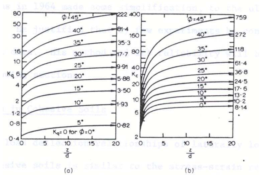
Fig. (2-3) Lateral Resistance Factors K_q and K_c (Brinch Hansen, 1961)
