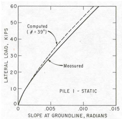
Fig. (3-16) Comparison between Measured Results of Mustang Island Tests and Results Computed with Proposed Criteria; Pile 1 Slope at Ground Line (Reese, 1974)
