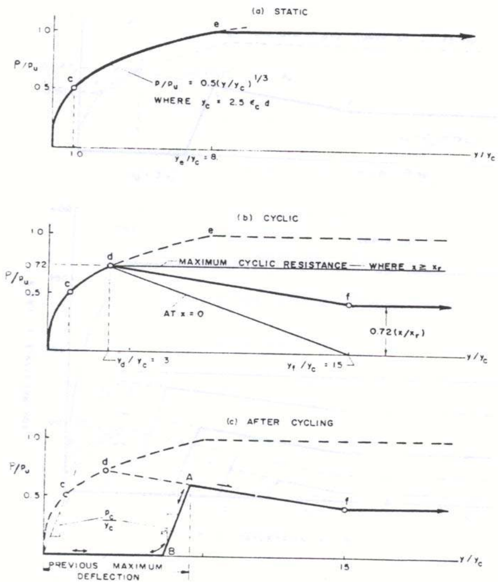
Fig. (3-12) Criteria for Predicting p-y Curves for (a) Short-term static loading, (b) Equilibrium under initial cyclic loading, and (c) Reloading after cycling (Matlock, 1970)
