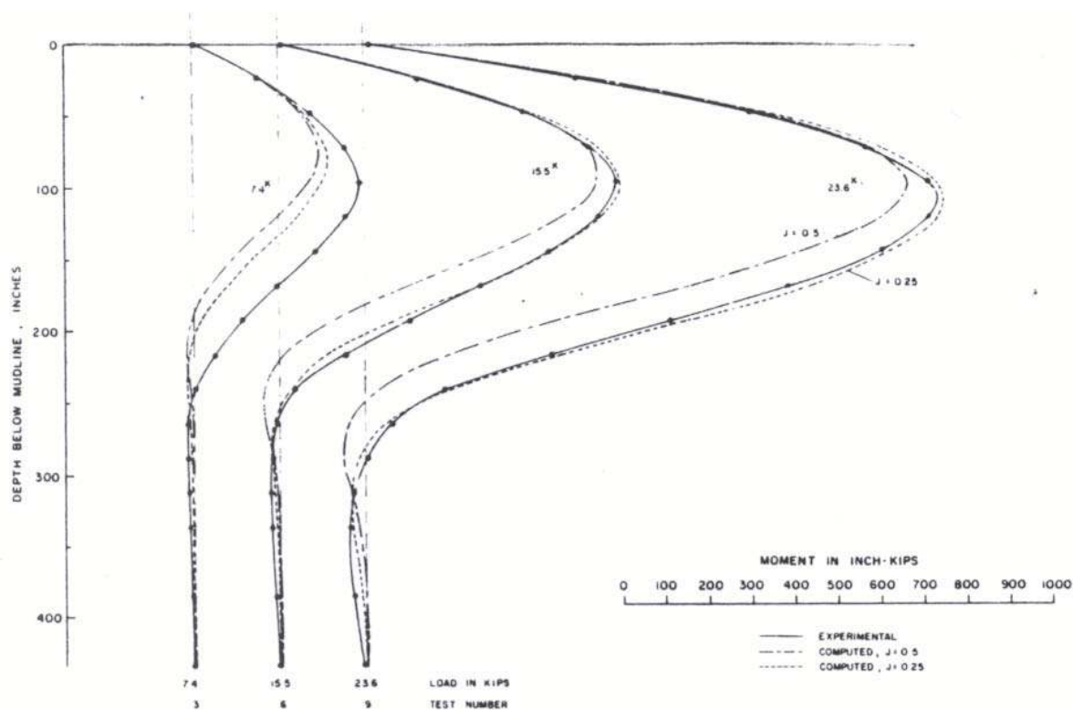
Fig. (3-25) Comparison of Computed and Experimental Results for Lake Austin Free-head Static Tests (Matlock, 1970)
