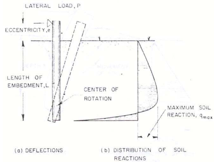
Fig. (2-13) Failure Mode of a Short, Free-Headed Pile (Broms, 1964a)
