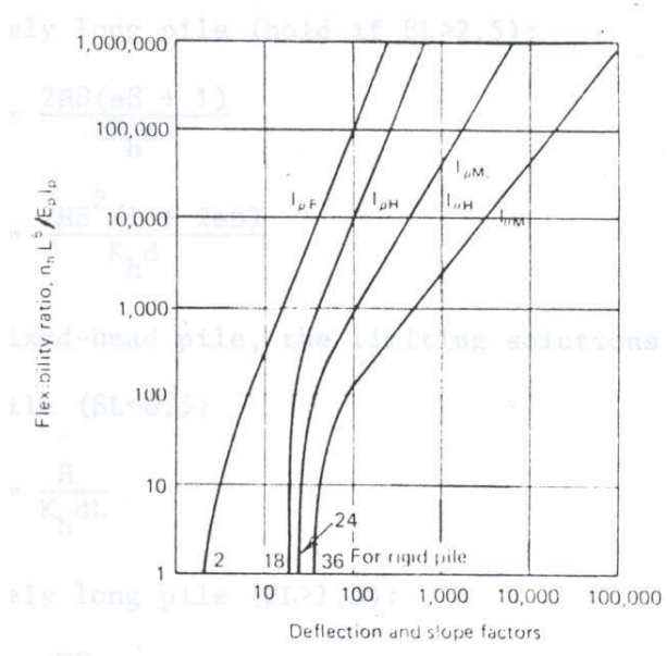
Fig. (2-22) Top Deflection and Rotation for Lateral Loads on Vertical Piles for k_h Proportional to Depth (Barber, 1953)
