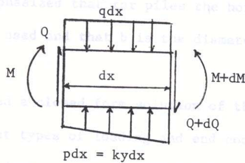
Fig. (1-1) Equilibrium Forces on an Element (Hetenyi, 1942)
