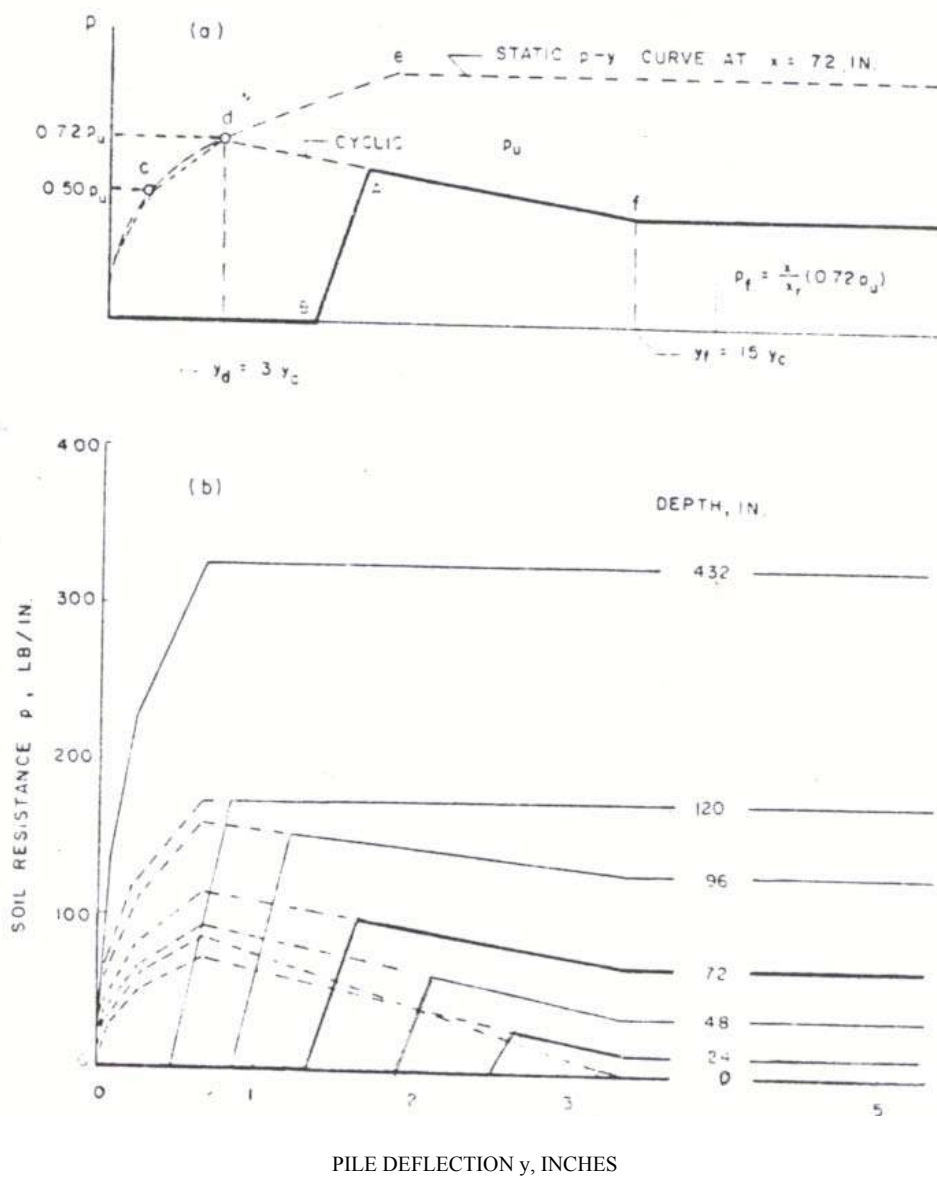
Fig. (3-13) Force-deformation Curves Predicted for Reloading after Prior Cyclic Loading to 13.5 kips, (a) Typical construction, (b) Complete family of curves (Matlock, 1970)
