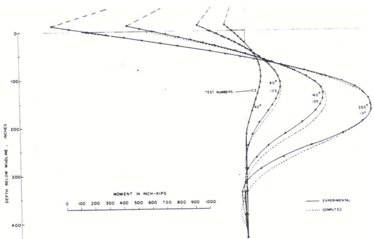
Fig. (3-23) Predicted Bending Moments for Sabine Restrained-head Static Loadings, Compared with Experimental Results (Matlock, 1970)
