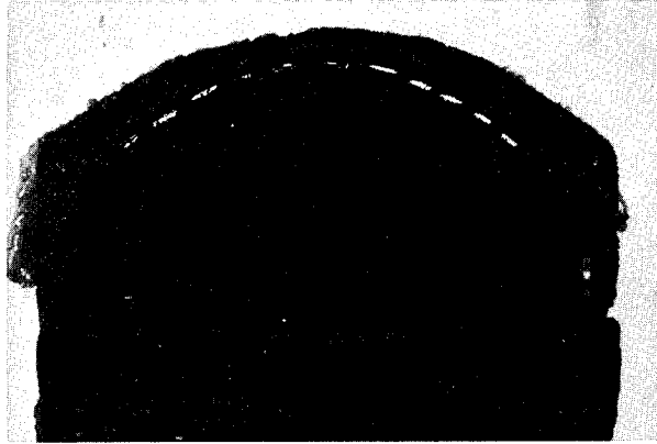
(a) Run 5; K = 0.232 ; p_{t,2} = 0.136 atm; H_0 = 0.427 kg/m 2 -sec; run time 45 sec.
