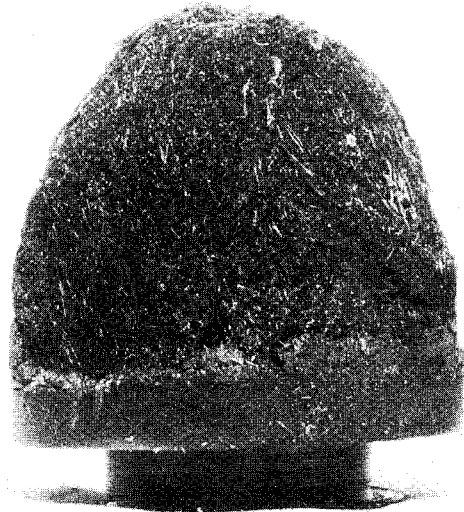
(b) Run 28; K = 0.118 ; p_{t,2} \approx 5 atm; run time 2 sec; H_0 = 3.09 kg/m 2 -sec.
