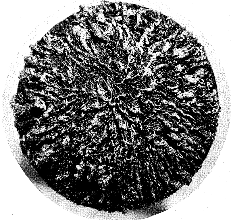
(a) Run 9; H_0 = 0.710 \text{ kg/m}^2\text{-sec} ; run time 20 sec; r_n = 1.3 \text{ cm} .
