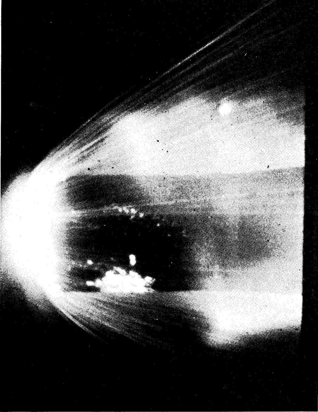
Figure 5.- Typical model spallation during test run in severe environment.
