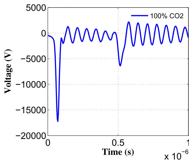
Figure 2. Oscilloscope of the voltage applied to the reactor for pure \text{CO}_2 .
