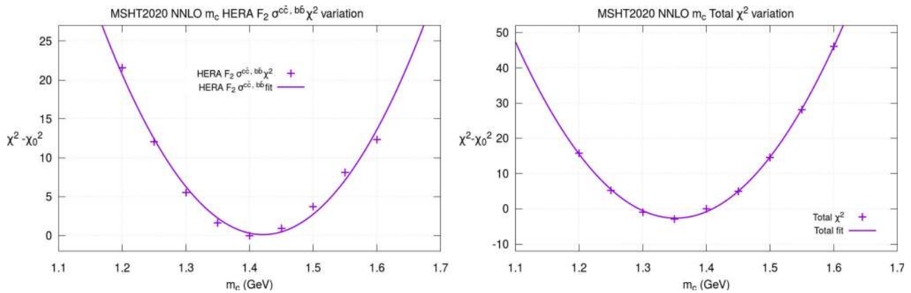
Fig. 16 The quality of the fit versus the quark mass m_c at NNLO with \alpha_S(M_Z^2) = 0.118 for (left) the reduced cross section for charm and bottom production \tilde{\sigma}^{c\bar{c}(b^{\prime})} for the combined H1 and ZEUS data and (right) the full global fit
