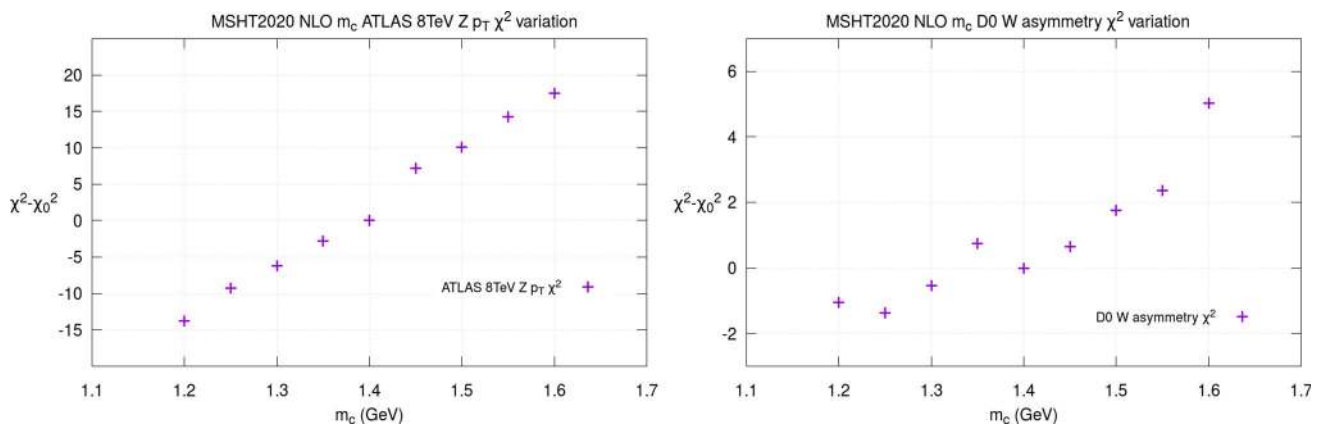
Fig. 15 The quality of the fit versus the quark mass m_c at NLO with \alpha_S(M_Z^2) = 0.118 for (left) the ATLAS 8 TeV Z p_T data and (right) the D\bar{0} W asymmetry data
