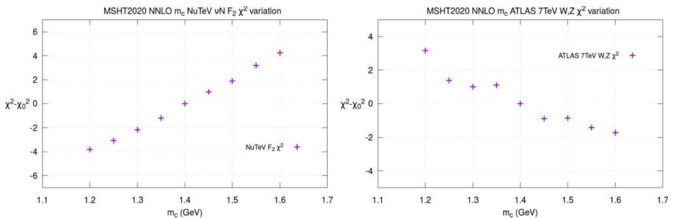
Fig. 19 The quality of the fit versus the quark mass m_c at NNLO with \alpha_S(M_Z^2) = 0.118 for (left) the NuTeV F_2(x, Q^2) data and (right) the ATLAS 7 TeV W, Z data
