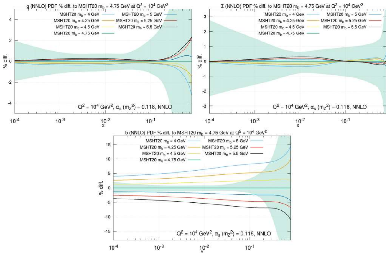
Fig. 26 The m_b dependence of the gluon, light-quark singlet and bottom distributions at NNLO for Q^2 = 10^4 \text{ GeV}^2 , compared to the standard MSHT20 distributions with m_c = 1.4 \text{ GeV} and m_b = 4.75 \text{ GeV}
