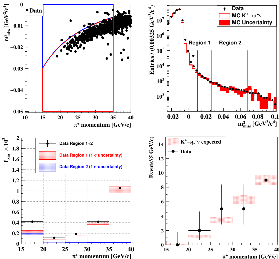
Figure 15. Top left: distributions of the PNN-triggered events in the (\pi^+ momentum, m_{\text{miss}}^2 ) plane after the PNN selection in the \mu\nu (red contour) and control m_{\text{miss}}^2 (blue contour) regions. The control region is used only for validation of the background estimation. Top right: reconstructed m_{\text{miss}}^2 distribution of the K^+ \rightarrow \mu^+\nu minimum-bias data events (full symbols, see text for details) integrated over the 15–35 GeV/c momentum range. The distribution of simulated K^+ \rightarrow \mu^+\nu decays is superimposed. Signal regions 1 and 2 are shown. Bottom left: the probability f_{\text{kin}} measured using the K^+ \rightarrow \mu^+\nu minimum-bias sample in bins of reconstructed \pi^+ momentum, separately for signal region 1 and 2 and combined (black symbols), and the corresponding statistical uncertainties. Bottom right: expected and observed numbers of background events from K^+ \rightarrow \mu^+\nu decays in the \mu\nu control region in \pi^+ momentum bins. The errors are statistically dominated.
