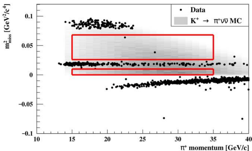
Figure 23. Reconstructed m_{\text{miss}}^2 as a function of \pi^+ momentum for PNN events (full symbols) satisfying the PNN selection, except the m_{\text{miss}}^2 and \pi^+ momentum criteria. The grey area corresponds to the expected distribution of SM K^+ \rightarrow \pi^+ \nu \bar{\nu} MC events (arbitrarily normalized). Red contours define the signal regions. The events observed in the signal regions are shown together with the events found in the background and control regions.
