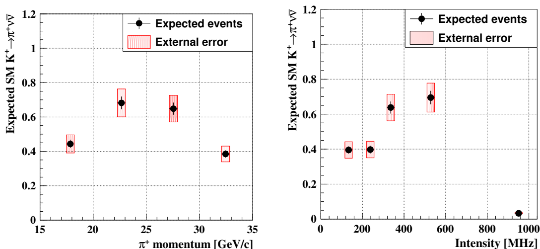
Figure 12. Number of expected Standard Model K^+ \rightarrow \pi^+\nu\bar{\nu} events in bins of \pi^+ momentum (left) and average beam intensity (right). The average beam intensity per bin, obtained from the K^+ \rightarrow \pi^+\pi^0 sample used for normalization, is plotted at the barycentre of the bin.
