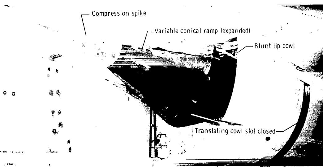
(b) Translating cowl slot closed; variable conical ramp expanded. E-21377
