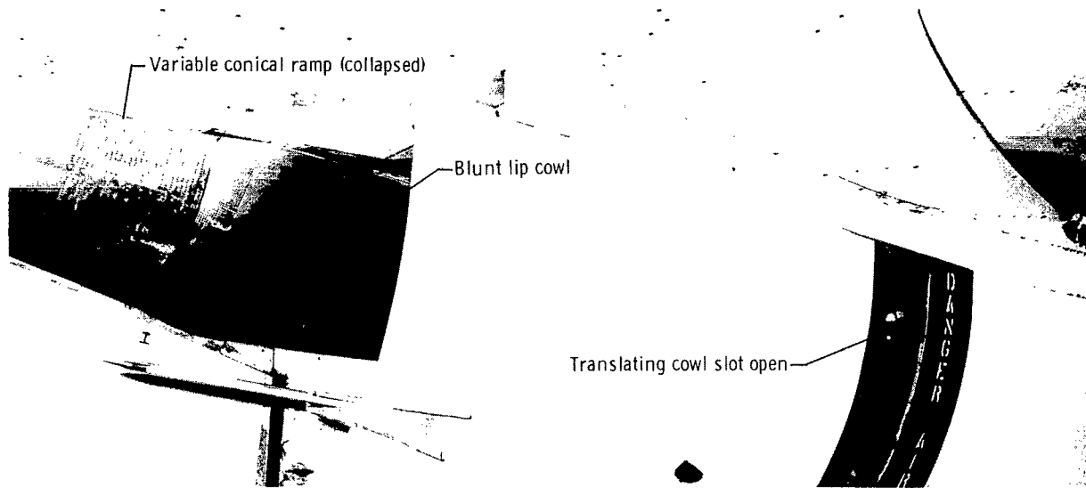
(a) Translating cowl slot open; variable conical ramp collapsed. E-21375
