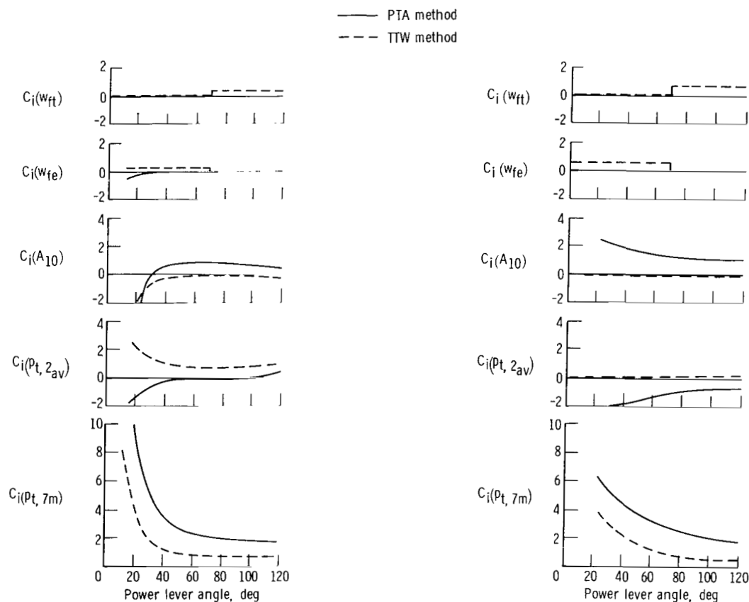
(a) Static conditions ( M_\infty = 0 ).
