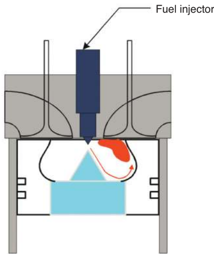
Figure 18 Schematic representation showing fuel trajectory and locally fuel-rich (stagnation) zone formed by piston bowl and cylinder head for late (near to TDC) SOI timings, wall-guided geometry.
