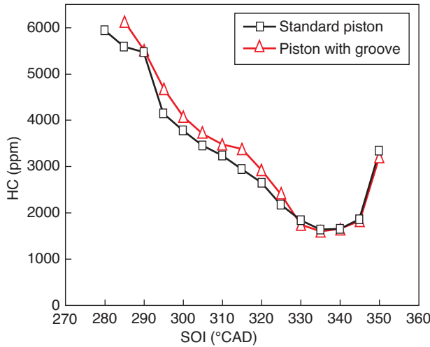
Figure 9 Comparison of HC emissions levels as a function of SOI timing showing effect of piston topland crevice volume, IMEP 4 bar, 45 %EGR, 1500 rpm, T_{int} = 60^{\circ}\text{C} , all-metal engine data, wall-guided geometry.
