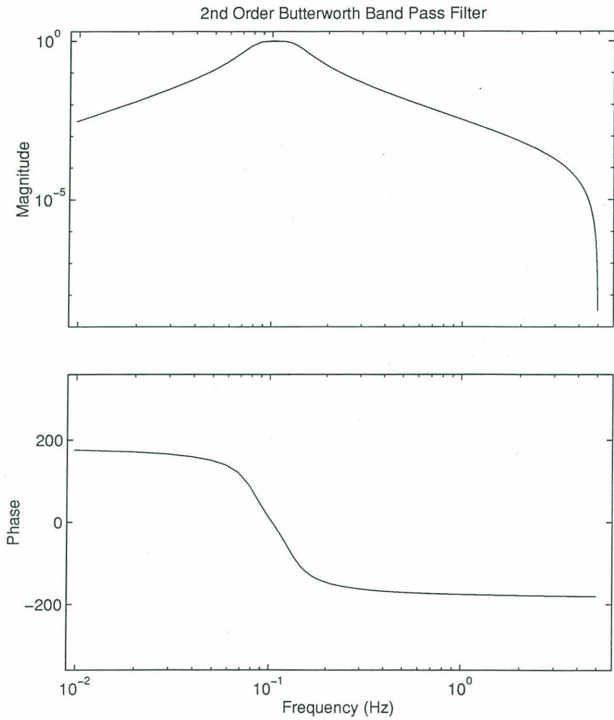
Figure 4.6 Illustration of the shape and phase of a 2nd order band-pass Butterworth filter, typical of those used in the analysis. The band-pass region is centered around the dominant wave frequency.
