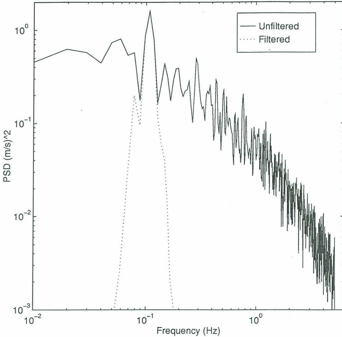
Sonic2 W-Velocity Spectra
