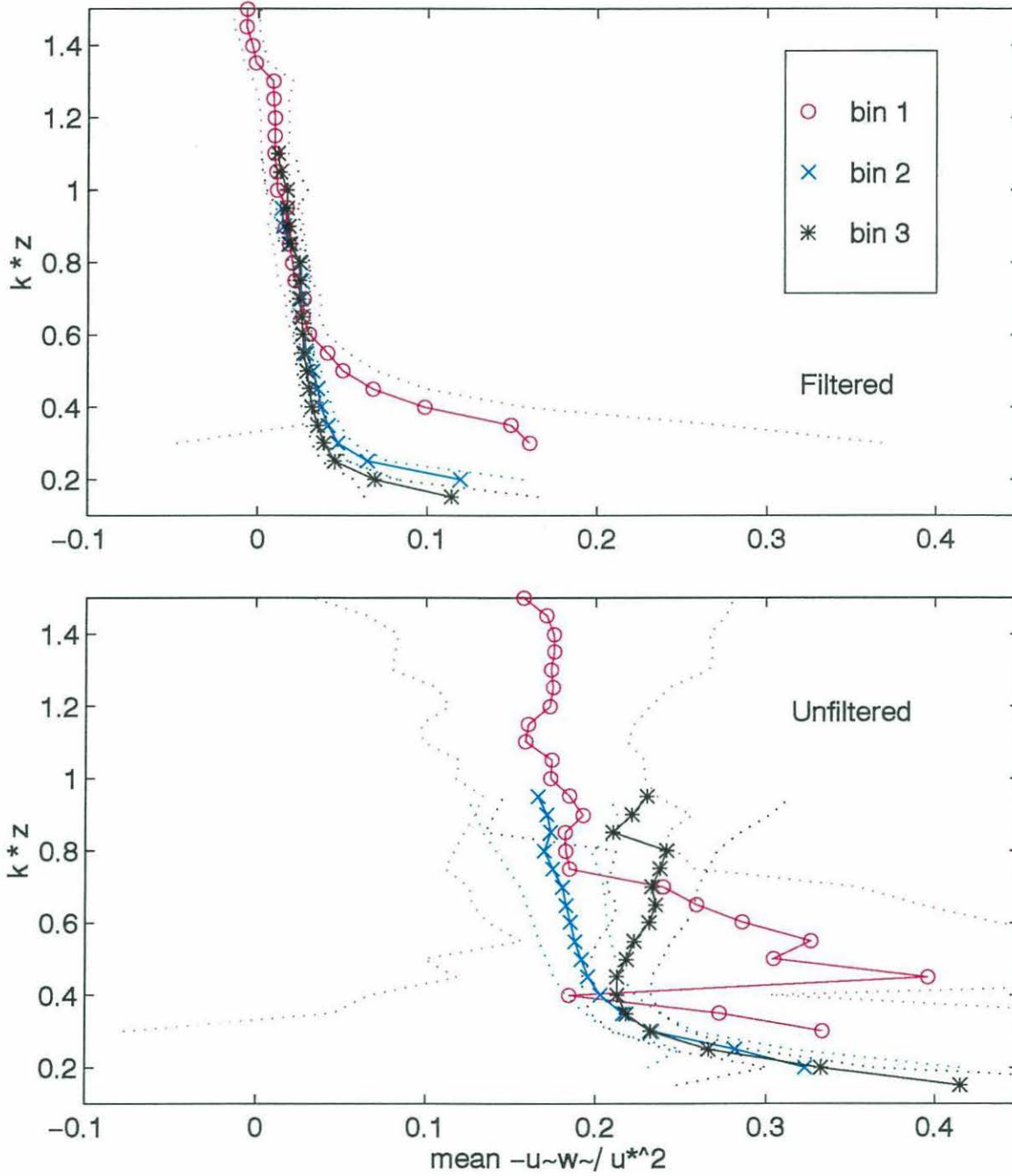
Wave-Induced Momentum Flux, sonic5234
