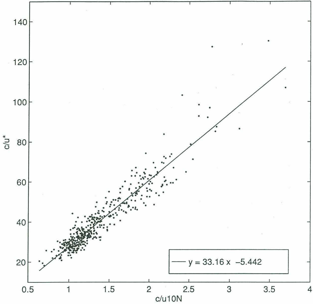
Comparison of Two Wave Age Parameters
