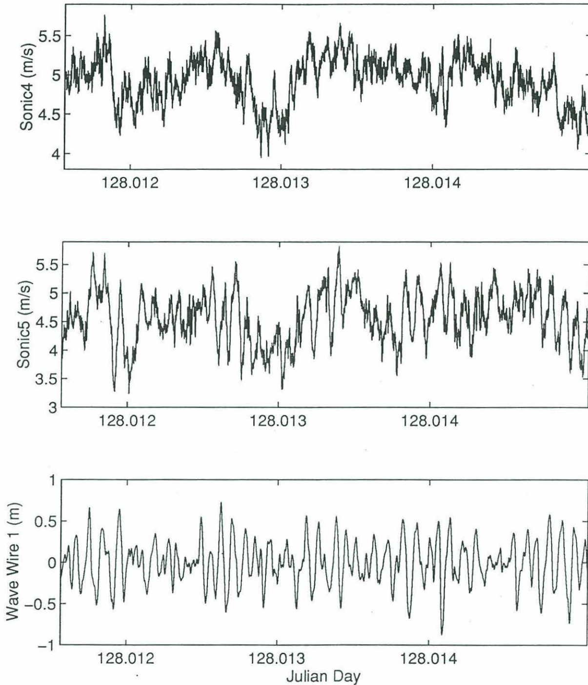
Figure 2.4 Time series of horizontal wind velocity from the upper (sonic 4, at 18.12 m above sea level) and lower (sonic 5, at 3.9 m) levels of sonic anemometers. Both show a strong correlation with the time series of the underlying wave field (wave wire 1). The decrease in wave heights just before day 128.013 is accompanied by a corresponding drop in horizontal wind velocities at both heights.
