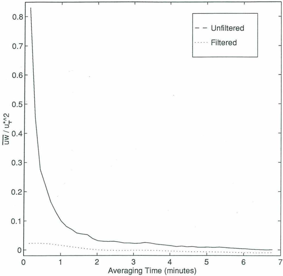
Turbulent Fraction of Total Flux Remaining after Phase Averaging
