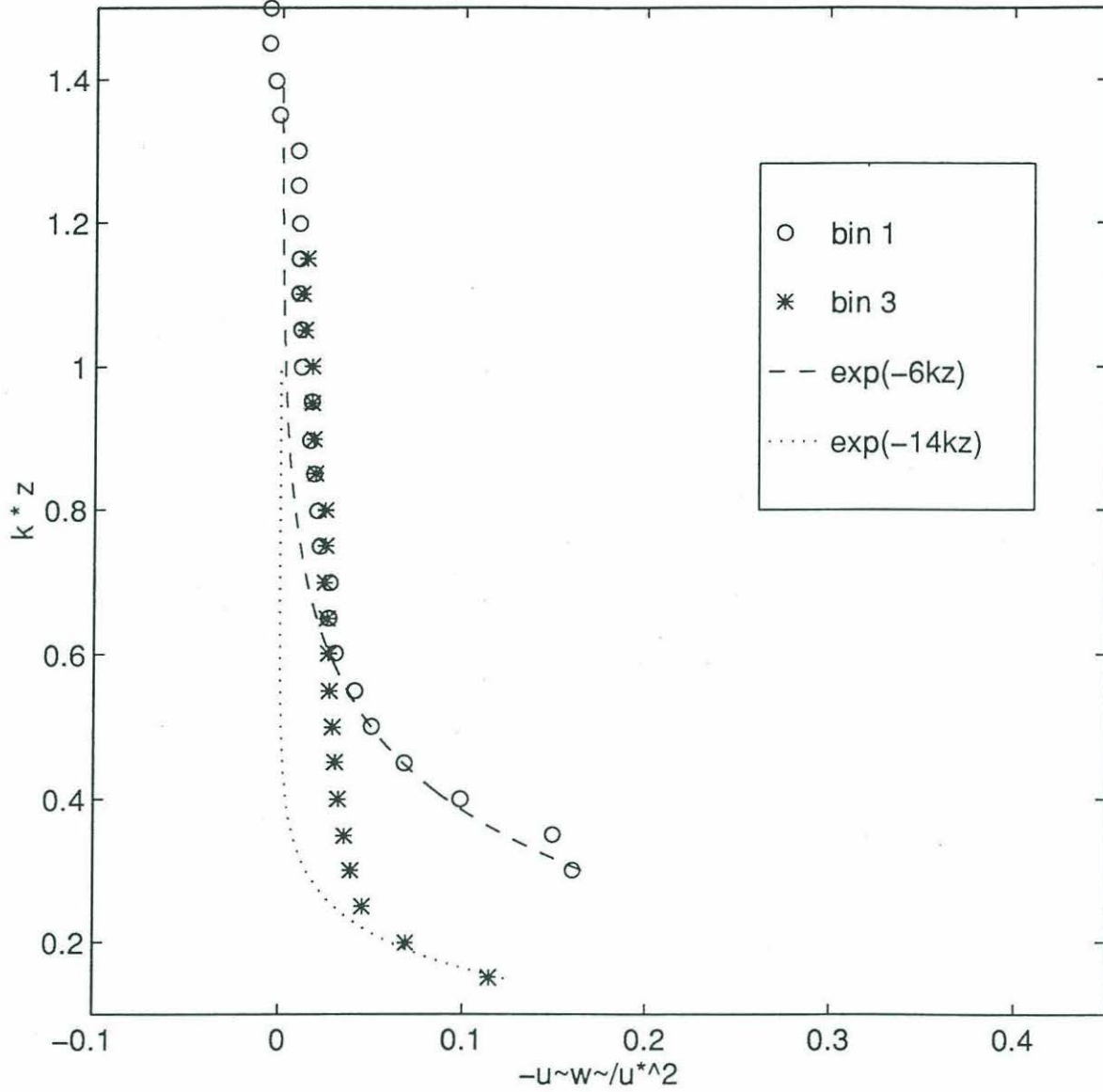
Wave-Induced Momentum Flux, with Parameterization
