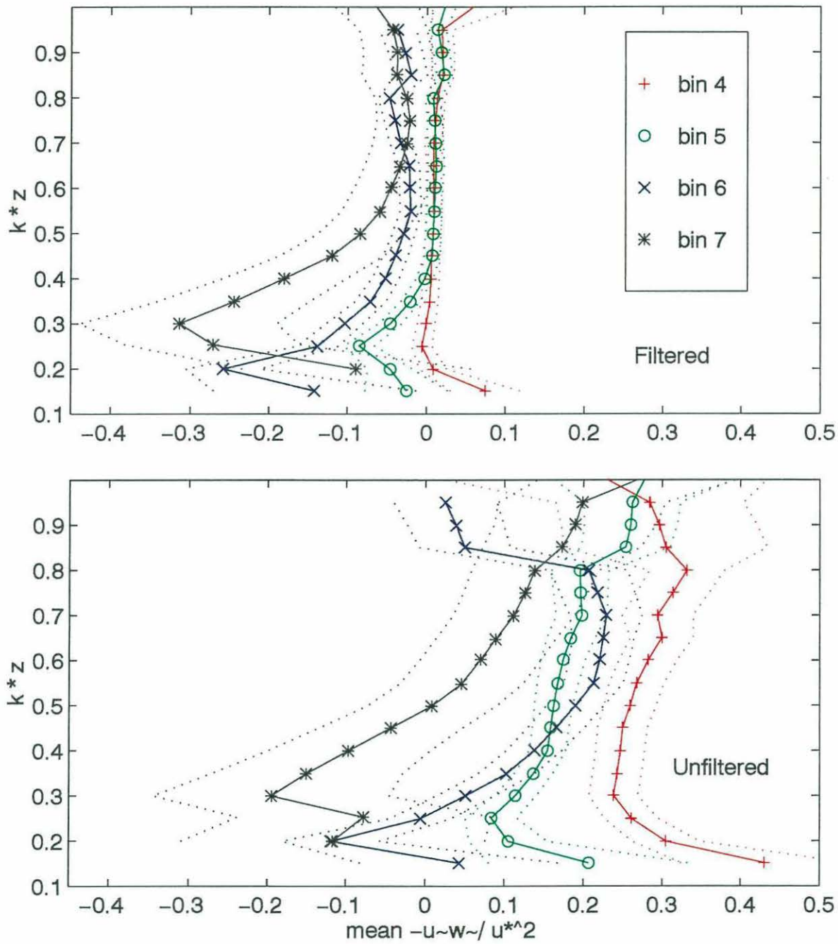
Figure A.4 Profiles of wave-induced momentum flux for bins 4-7 using filtered (top) and unfiltered (bottom) wind velocities in the analysis of the original results.
