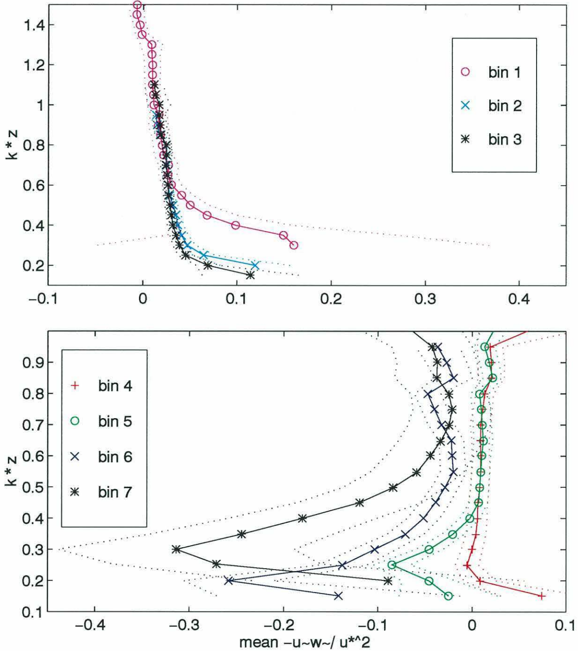
Figure 5.3 Results of bin averaging profiles of wave-induced momentum flux by wave age. The first three bins, corresponding to developing waves, show a transfer of atmospheric momentum to the ocean wave field. The flux is nearly zero for the fully developed sea and becomes negative indicating a transfer of momentum from the waves to the atmosphere for decaying seas. The wave age groups corresponding to each bin are listed in table 5.1.
