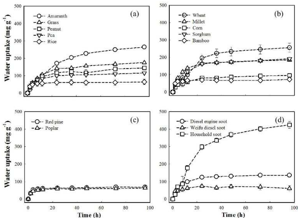
Figure 4. Sorption kinetics of water vapor plotted as water uptake ( \text{mg g}^{-1} ) vs. time (h) at 94 % relative humidity. (a) Subgroup 1 of herbal BCs. (b) Subgroup 2 of herbal BCs. (c) Woody BCs. (d) Soot. Error bars represent standard variations from duplicate samples.
