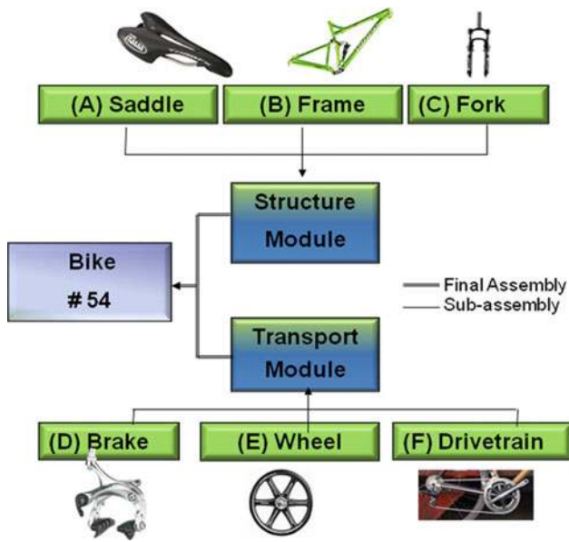
Fig. 5 Two-module product architecture
