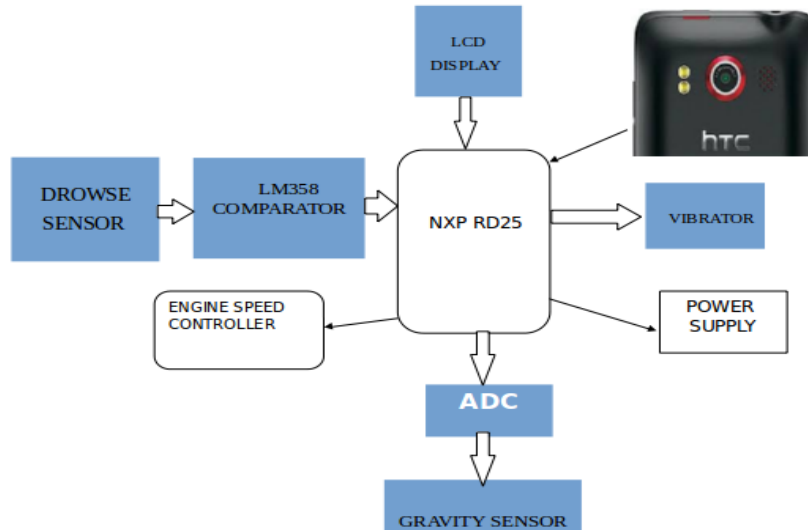
Fig.1 Block diagram of implemented prototype
