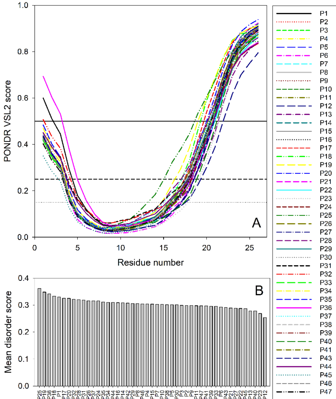
Figure 5: Analysis of intrinsic disorder predisposition of 47 T-ORF8 proteins: (A) Disorder profiles generated using the PONDR-VSL2 disorder predictor. Three thresholds of predicted disorder scores (PDSs) are shown, 0.15, 0.25, and 0.5, which are used for the classification of protein residues as highly disordered ( PDS \geq 0.5 ), flexible ( 0.25 \leq PDS < 0.5 ), moderately flexible ( 0.15 \leq PDS < 0.25 ) and mostly ordered ( PDS < 0.15 ). (B) Ranking 47 T-ORF8 proteins based on their mean disorder scores.
