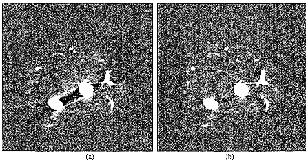
Fig.3 Reconstructed rat lung image at slice location 90 (display window width=1500, window level=100) (a) original image (b) corrected image
