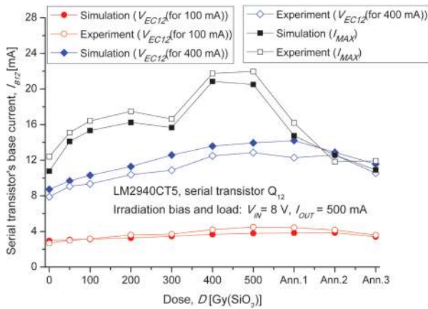
Figure 6: Variations of the serial transistor's base current as a function of the total ionising dose and type of annealing: comparison between simulation and experimental results. Bias conditions during irradiation: V_{IN} = 8\text{ V} , I_{OUT} = 500\text{ mA} .
