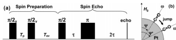
Figure 1. (a) Schematic diagram of the pulse sequence, the S-shape sequence. (b) Schematic diagram of CO surface diffusion altering the ^{13}\text{C} Larmor frequency ( \omega ).
