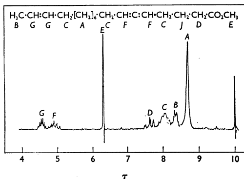
Fig. 3. Nuclear-magnetic-resonance spectrum of methyl lamellenate. Experimental details are given in the text. The signal due to protons labelled J is obscured by signal B or C .
