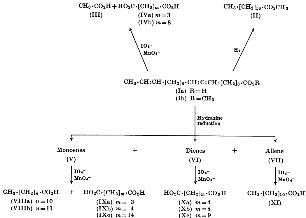
Scheme 1.
