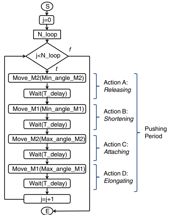
Figure 7. Flow chart of the controlling algorithm. N_loop is the number of pushing actions the robot will perform; Min_angle is the minimum angle the servos will be driven, i.e. Min_angle = 0 rad for both servos. Max_angle is the maximum angle the servos will be driven, i.e. will be \frac{2\pi}{3} rad for M1 and \pi rad for M2. The function Move() sends the command to the servos and the function Wait() introduces a delay of time T_delay between two commands. The total time of the various actions from A to D is defined as the pushing period. Varying the delays we will change the period time. For the sequences single servo and reduced friction we use only the first servomotor (M1), so the code relative to actions A and C was deleted.
