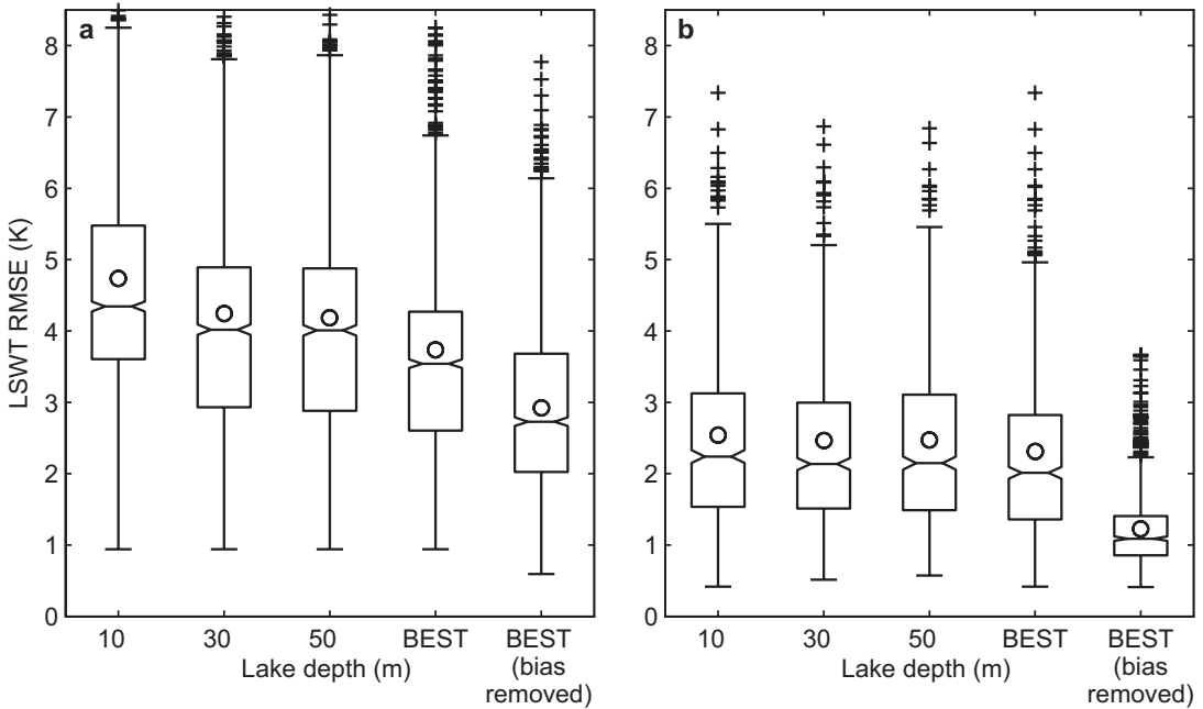
Fig. 2. Root mean square error distributions of the model vs. MODIS observations of lake surface-water temperature (LSWT, WL) of (a) high latitude (latitude > 40^\circ ) lakes, and (b) low latitude (latitude < 40^\circ ) lakes for all ERAI grid-boxes with more than 10% of available remotely sensed LSWTs data in the period January 2001 to December 2005. Separate statistics are given, since the dependence of the lake thermodynamics on the latitude is very pronounced due to the impact of freezing in high-latitude lakes. Distributions of RMSE are presented as function of lake depths (10, 30 and 50 m) and BEST (lake depth that minimizes the RMSE for each grid point). The rightmost “BEST (bias removed)” give results with the model-observations bias removed before computing RMSE. The boxes have horizontal lines at the lower quartile, median, and upper quartile, and outliers are data with values beyond 1.5 times the inter-quartile range indicated with ‘+’. Open circles are the means. Remotely-sensed LSWTs missing data are due to (i) cloud covered pixels, (ii) frozen lakes (the retrieval algorithm can only be applied for open water surfaces), and (iii) other errors in the retrieval algorithm.
