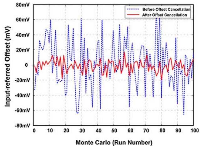
Fig. 10 Monte Carlo simulation of the offset in comparator (before and after offset cancellation)
