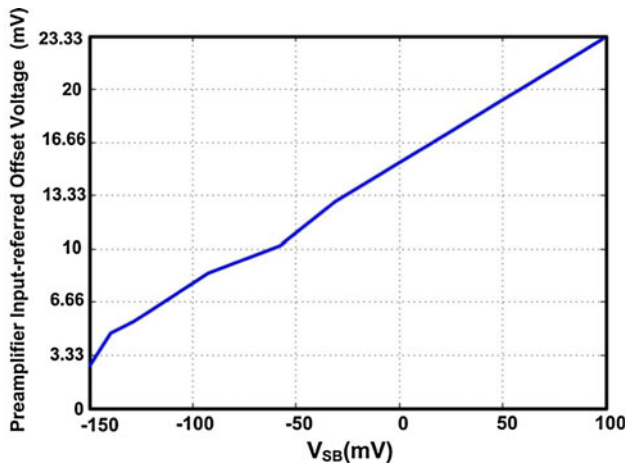
Fig. 8 Preamplifier input-referred offset voltage versus source-body variation of the corresponding input transistor
