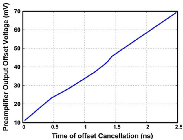
Fig. 9 preamplifier input-referred offset voltage versus time of offset cancellation
