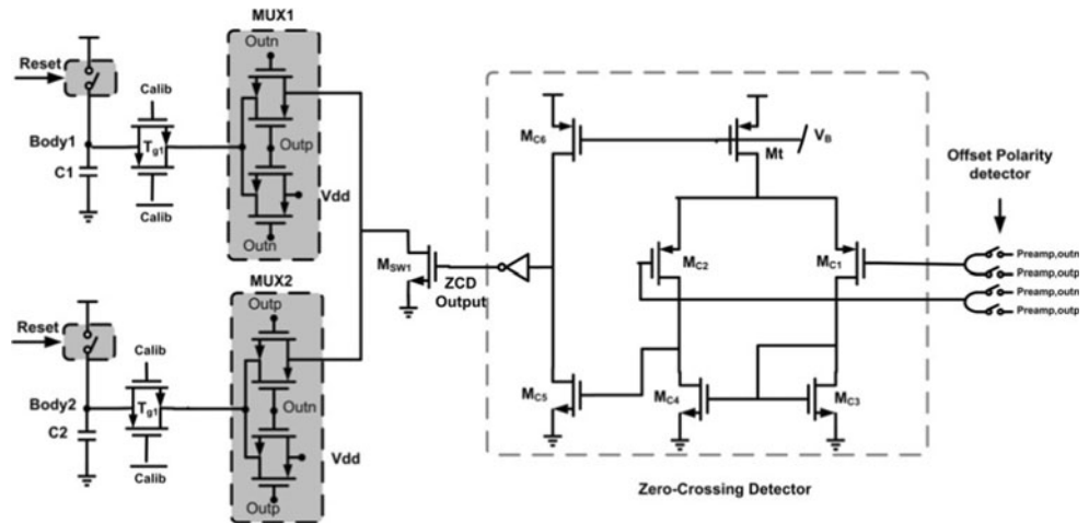
Fig. 5 The schematic of the offset cancellation network
