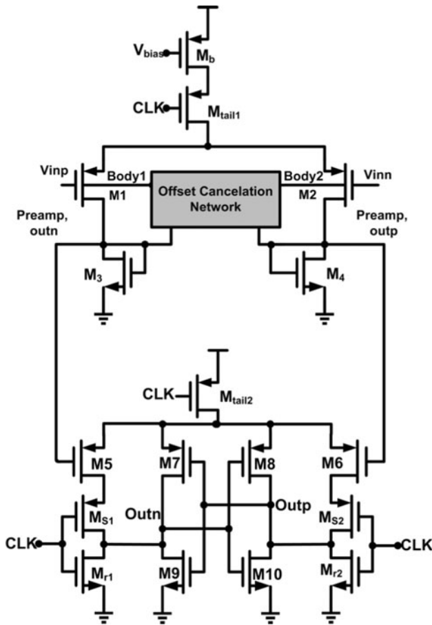
Fig. 1 The schematic of the comparator: preamplifier and dynamic latch
