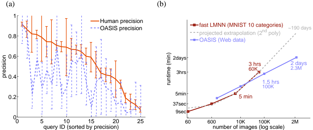
Figure 1: (a) Precision of OASIS and human evaluators, per query, using rankings of all (remaining) human evaluators as a ground truth. (b) Comparison of the runtime of OASIS and fast-LMNN[17], over a wide range of scales. LMNN results (on MNIST data) are faster than OASIS results on subsets of the web data. However LMNN scales quadratically with the number of samples, hence is three times slower on 60K images, and may be infeasible for handling 2.3 million images.
