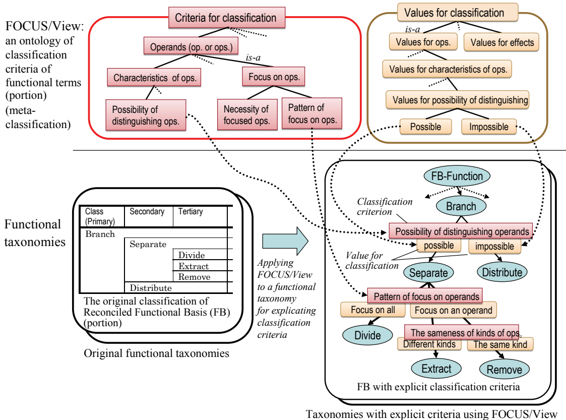
Figure 1. An overview of FOCUS/View with Reconciled Functional Basis (FB) as an example of a target taxonomy.
