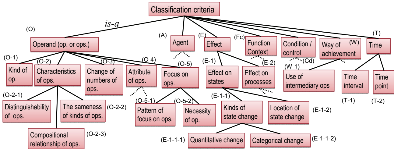
Figure 3. Classification criteria defined in FOCUS/View (portion).
