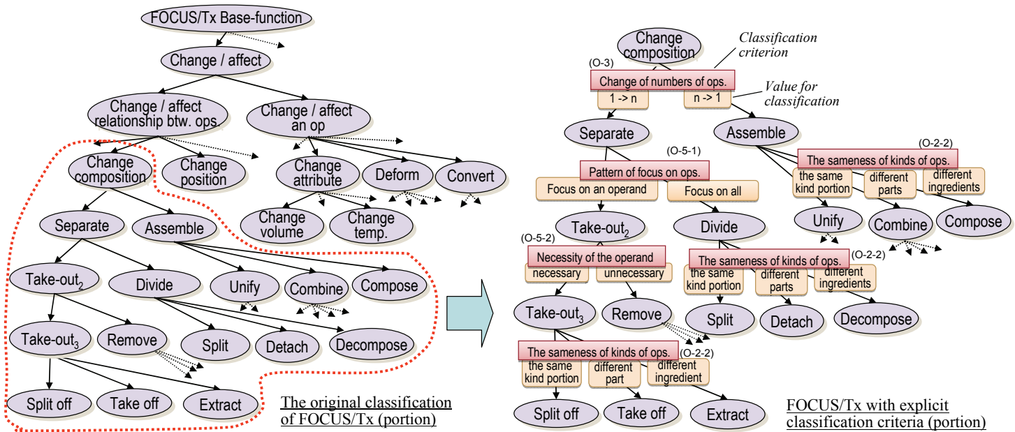
Figure 5. Classification criteria of FOCUS/Tx (Portion)
