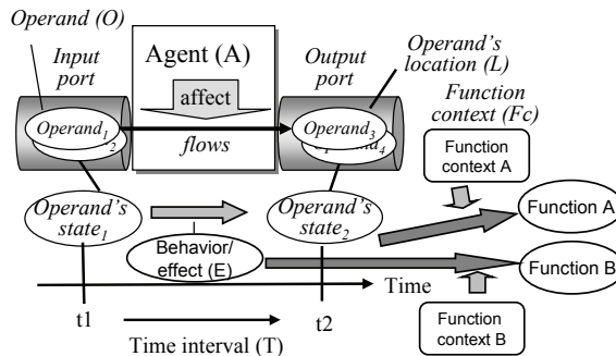
Figure 2. The base-model of function for FOCUS/View
