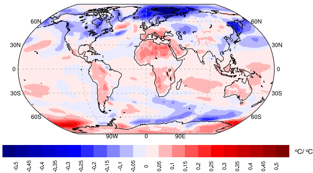
Figure 9. Ensemble mean annual average difference in ^{\circ}C/^{\circ}C in the ratio of local/global linear trend over the 21st century (2006–2100) between rcp8.5 and rcp4.5.
