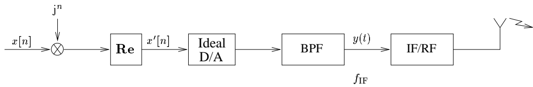
(b) System model
