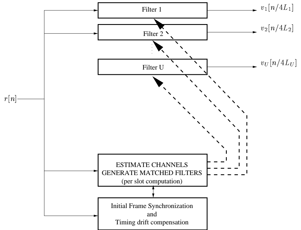
Figure 10: Basic RX structure
