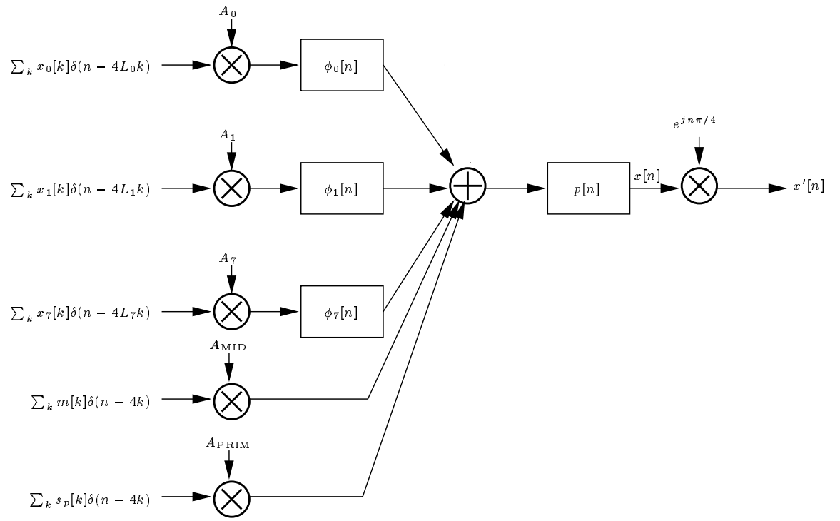
Figure 6: Basic TX structure
