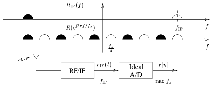
Figure 9: Receiver front-end
