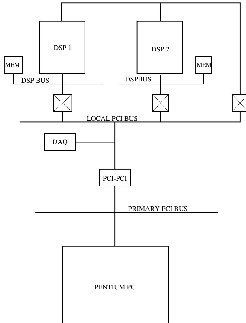
Figure 4: Embedded DSP Architecture
