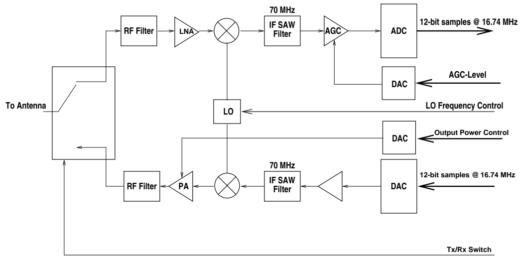
Figure 2: RF Front-end
