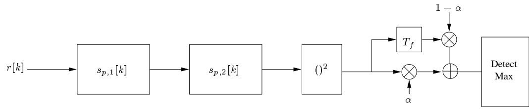
Figure 11: Primary Synchronization Processing
