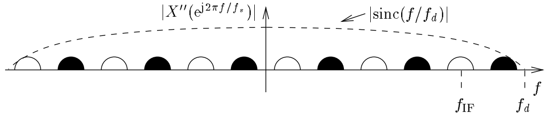
(b) D/A frequency response with up-sampling
