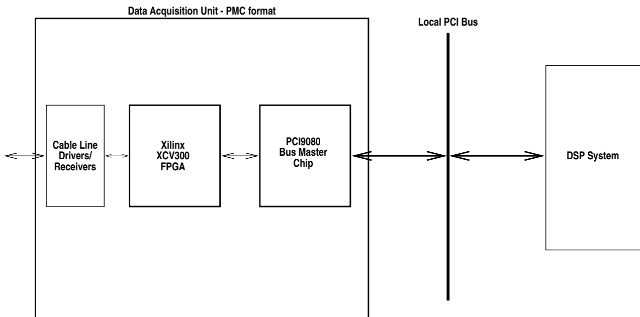
Figure 3: Data Acquisition Unit
