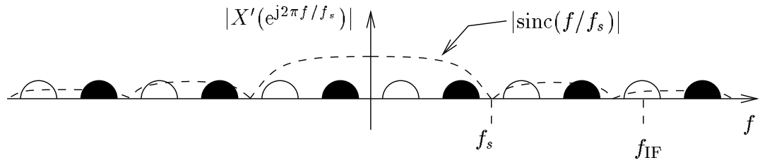
(a) D/A frequency response without up-sampling
