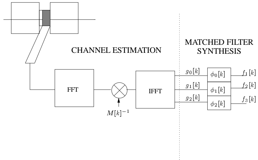
Figure 12: Channel Estimation and Matched Filter Synthesis
