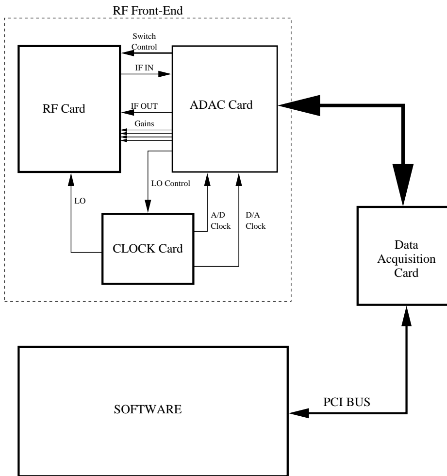
Figure 1: System Architecture
