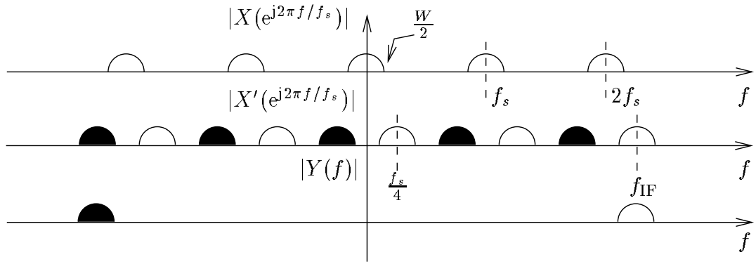
(a) Spectrum of x[n] , x'[n] , and y(t) with the integer \ell = 2 and the sign (+) chosen in (4)
