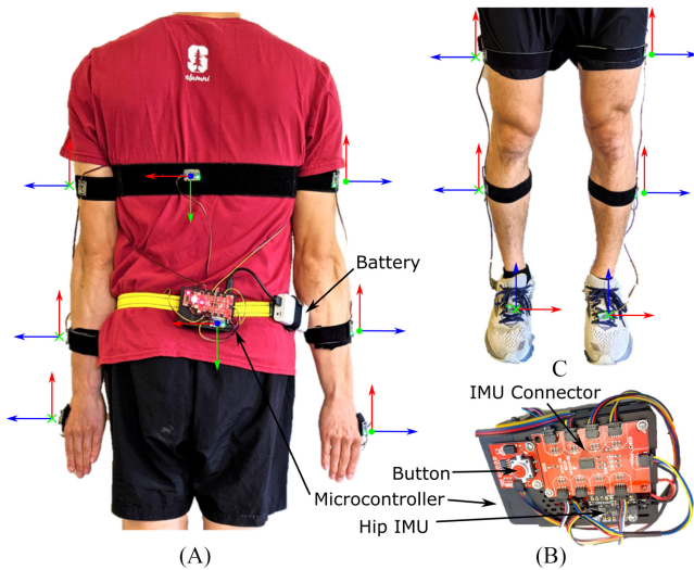
Fig. 1. The components and default IMU orientations of the OpenSenseRT System. (A) An IMU on the pelvis is required and acts as the base in order to compute the relative orientation of other sensors. The OpenSenseRT System accommodates a variable number of additional IMUs to customize which kinematics are measured. To monitor movement of the upper body, three IMUs may be placed on each arm (on the upper arm, forearm, and hand). An additional IMU can be placed on the torso. The orientation frame with axes shown in red, green, and blue is used to orient the x , y , and z axes defined on each IMU. These individual body frames should align with the world reference frames of the fore-aft, mediolateral, and vertical axes, while the subject's joint segments are aligned in a neutral standing (or other known) position. (B) The lower-limb IMU placements also require the pelvis IMU as a base and can include up to three IMUs on the thigh, shank, and foot of each leg. OpenSenseRT allows for 1 to 14 of these IMUs to be sampled in a custom configuration. (C) A zoomed in view of the system components shows the microcontroller, battery, button (for starting and stopping recordings), IMU connector, and pelvis IMU.
