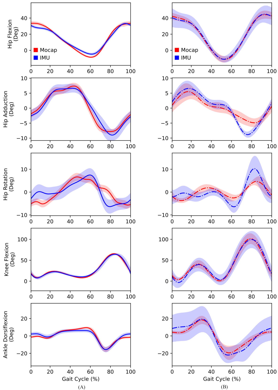
Fig. 3. Lower-limb joint kinematics computed with the OpenSenseRT system compared to optical motion capture. (A) Joint kinematics during walking at 1.25 m/s were computed in real-time at 30 Hz with the IMU system for five subjects. The error bands represent one standard deviation of the RMSE across all subjects. (B) Joint kinematics during running at 4.0 m/s were computed offline (represented with the dash-dot line) at 100 Hz with the IMU system for a single subject. The error bands represent one standard deviation of the RMSE across all gait cycles for the single subject. Running requires a faster computation rate than the IMU system can perform consistently in real-time, although it can be analyzed in real-time over short bursts by using all cores.
