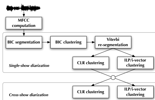
Figure 1: Diarization steps
