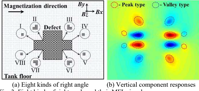
Fig. 3. Eight kinds of right angle and their MFL signal responses.
