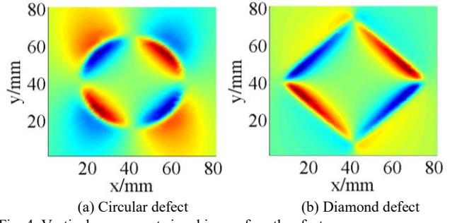
Fig. 4. Vertical component signal image for other features
