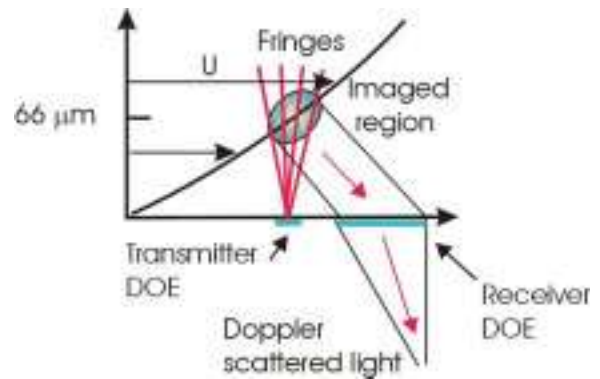
Figure 1 Schematic of the optical shear stress sensor principle of measurement.
