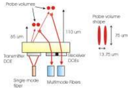
Figure 6 Design of the Dual Microvelocimeter with two probe volumes, one probe volume located at 65 \mu\text{m} and a second probe volume located at 110 \mu\text{m} above the surface of the sensor.
