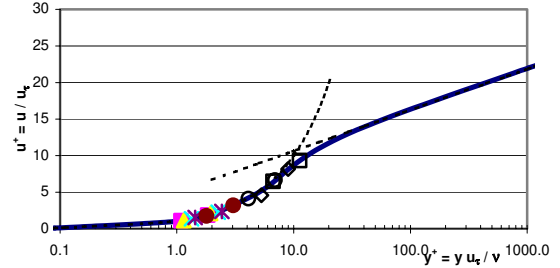
Figure 11 Spalding fit to dual velocity measurements using the Dual Velocity sensor
