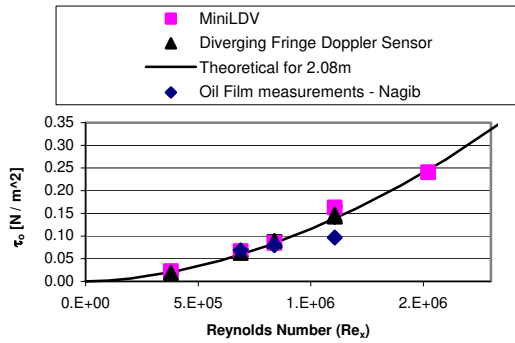
Figure 10 - Wall shear stress measurements obtained with the diverging fringe Doppler sensor compared to that obtained with the MiniLDV.
