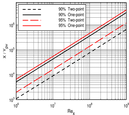
Figure 3 Accuracy of wall shear stress in a flat plate turbulent boundary layer based on two-point velocity data from probe volumes located at Y_{pv} and 2Y_{pv} . An empirical method is used to estimate the wall velocity gradient. To achieve the indicated level of accuracy, the conditions must lie above the corresponding line.
