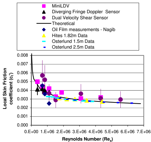
Figure 13 Comparison of local skin friction measurements obtained with the diverging Doppler sensor, the dual Velocity sensor, LDV, oil film, and additional results obtained by Österlund 9 and Hites 10 .
