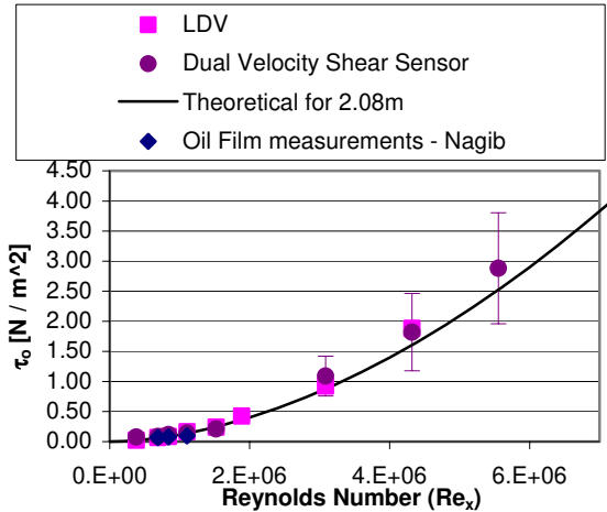
Figure 12 Wall shear stress measurements with the Mini LDV, the Diverging Doppler sensor and oil film interferometry.
