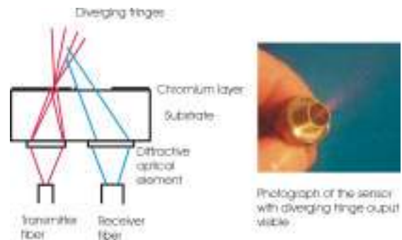
Figure 2 Diverging Fringe Doppler sensor design
