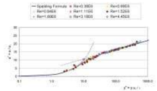
Figure 9 Turbulent velocity profiles measured in the 2’ wind tunnel
