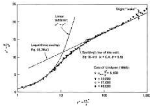
Figure 5 Mean velocity profile of a turbulent boundary layer from “Viscous Fluid Flow” by F. A. White.
