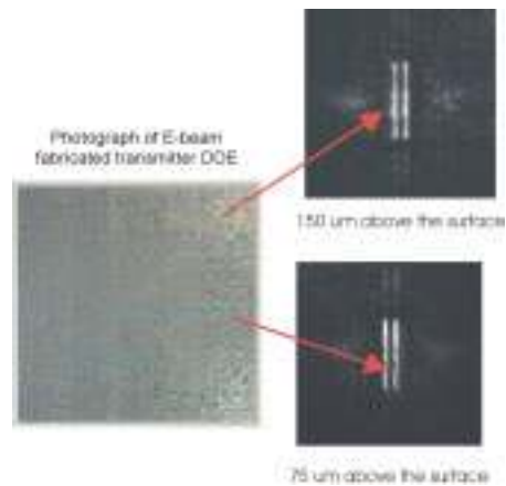
Figure 7 Photographs of the transmitter DOE and of the two probe volumes. The locations of the probe volumes are given for use in water.
