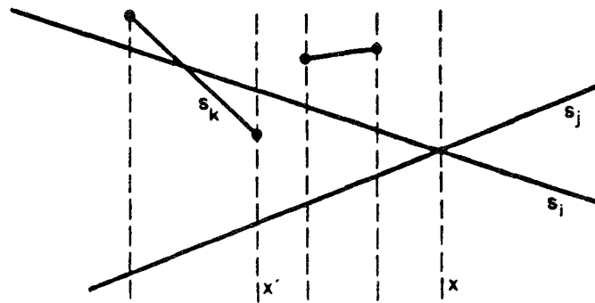
FIG. 2. We delete segment s_k from the cross-section when the vertical sweep-line process passes x' , the x -coordinate of its right endpoint. As we do this, segments s_i and s_j become adjacent and we discover that they are about to intersect.
