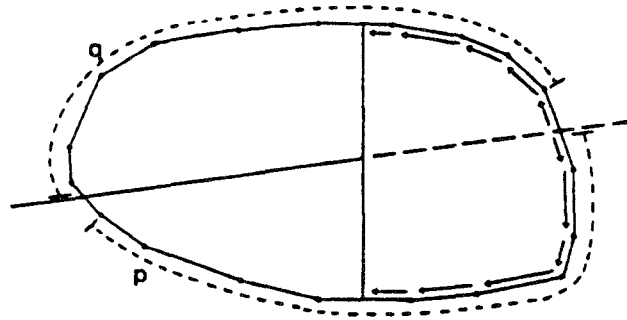
FIG. 6. A terminating region is cut into four pieces, rather than three. This causes no harm because the two right regions will never again be traversed. It is important that we do the second step (finding the endpoints of the stop) from right to left.
