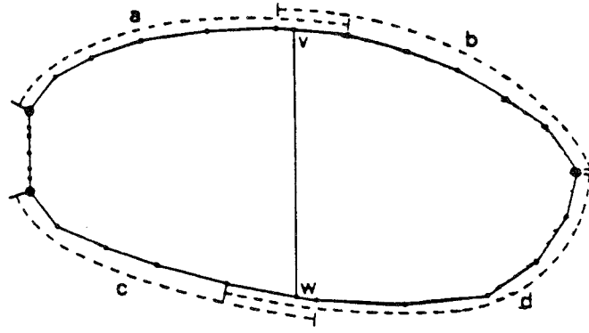
FIG. 36. Starting at v (or w , if the reader prefers), we perform a dovetailing traversal of the region in order to add the vertical edge from v to w .
