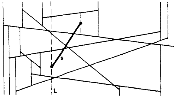
FIG. 9. Inserting a new segment.
