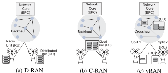
Fig. 1: RAN Architectures. (a) D-RAN places all functions at the BSs and transfers only the payload to EPC; (b) C-RAN places all functions at the cloud units; (c) vRAN selects possibly a different split for each BS, placing functions both at the DUs and CUs.
