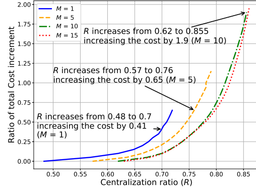
Fig. 12: Centralization R as a function of cost increment ( J^*/J )%: Plots correspond to different values of CU locations M = \{1, 5, 10, 15\} , and present mean values for all topologies by varying c_d \in [1, 10] and \lambda_m \in [50, 500] , creating 864 experiments.
