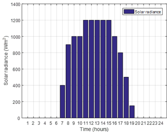
Figure 7: Solar irradiance
