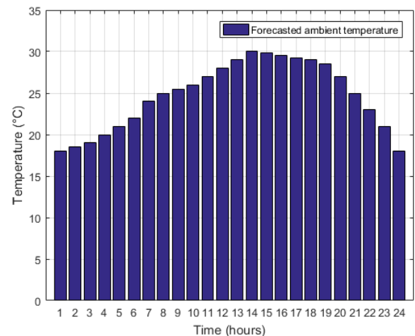
Figure 4: Forecasted temperature
