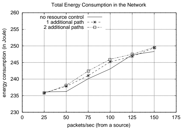
Fig. 11. Total energy consumption in the network
