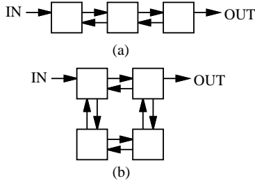
Fig. 7. Array topology and data input/output specification. (a) For 4th order Jaumann wave digital filter. (b) For 16 point FIR filter and 5th order wave elliptic digital filter.
