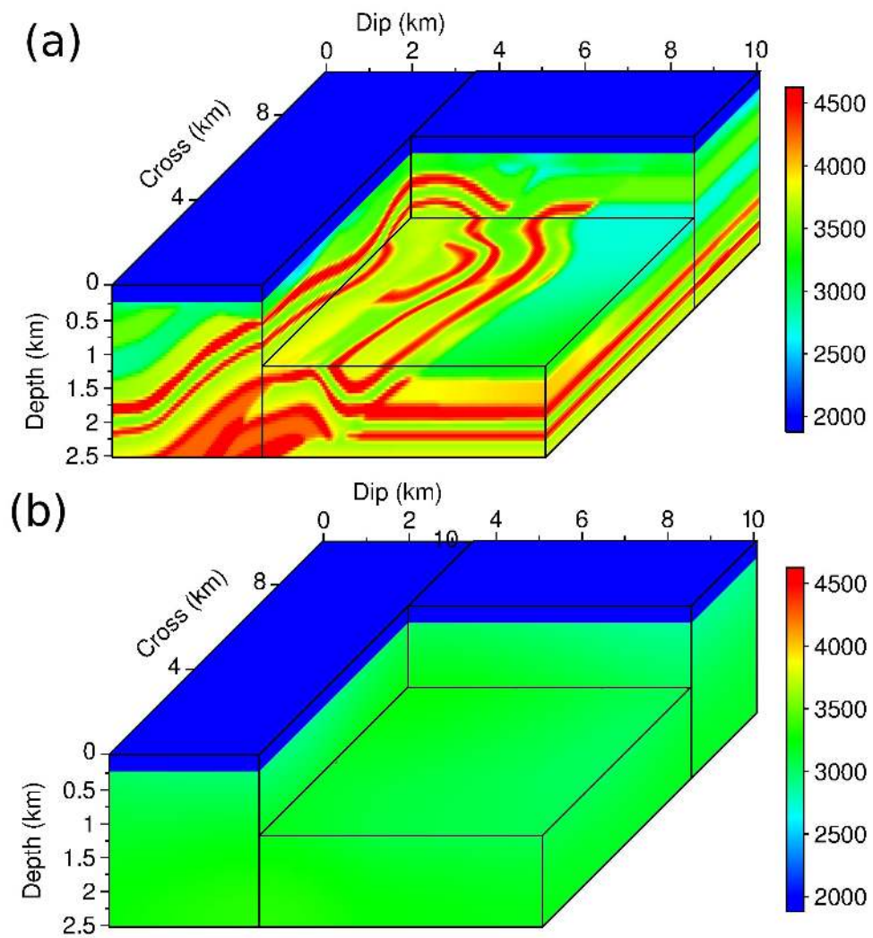
Figure 11. Exact (a) and initial (b) models used for the 3D SEG/EAGE overthrust case study.
