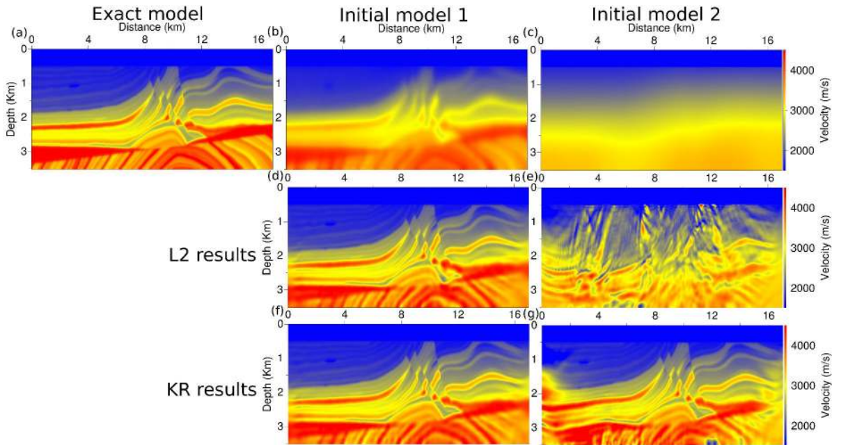
Figure 8. Marmoussi model case study. Exact model (a), initial model 1 (b), initial model 2 (c), results obtained with the L^2 distance starting from model 1 (d), from model 2 (e), results obtained with the KR distance starting from model 1 (f), from model 2 (g).
