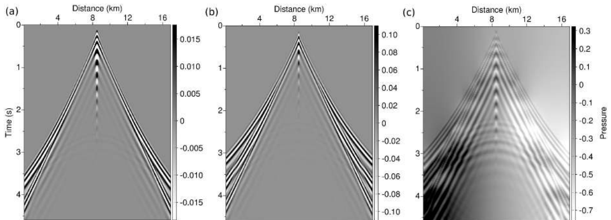
Figure 7. Observed data for the reference model (a). L^2 (b) and KR (c) residuals for the model v_{P,0} = 2250 \text{ m s}^{-1} , \alpha = 0.9 \text{ s}^{-1} .
