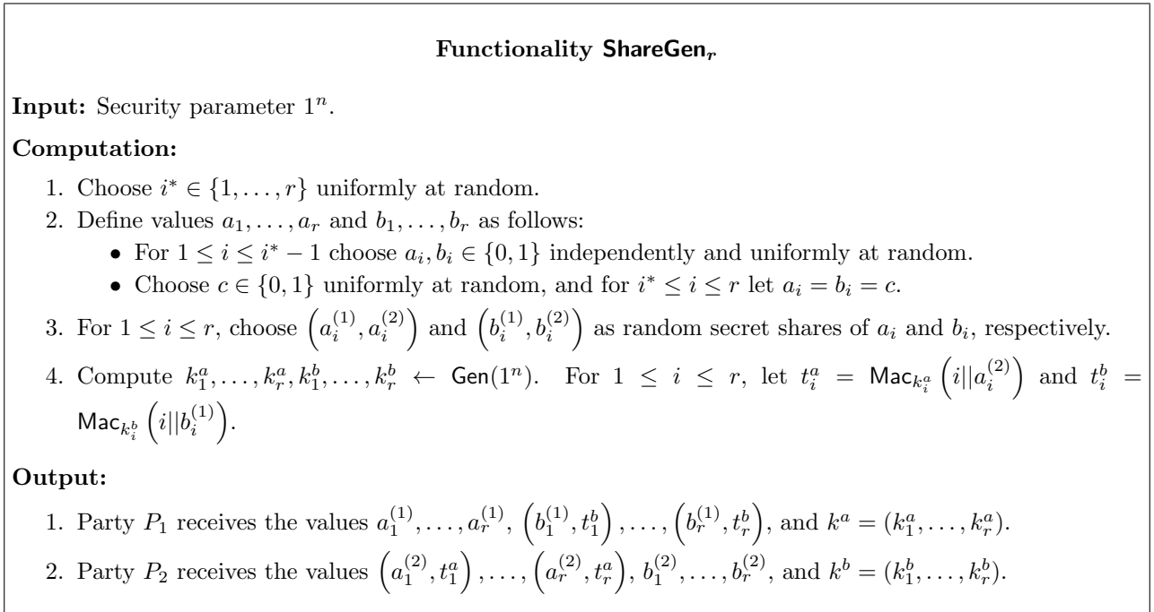
Figure 1: The ideal functionality \text{ShareGen}_r .
