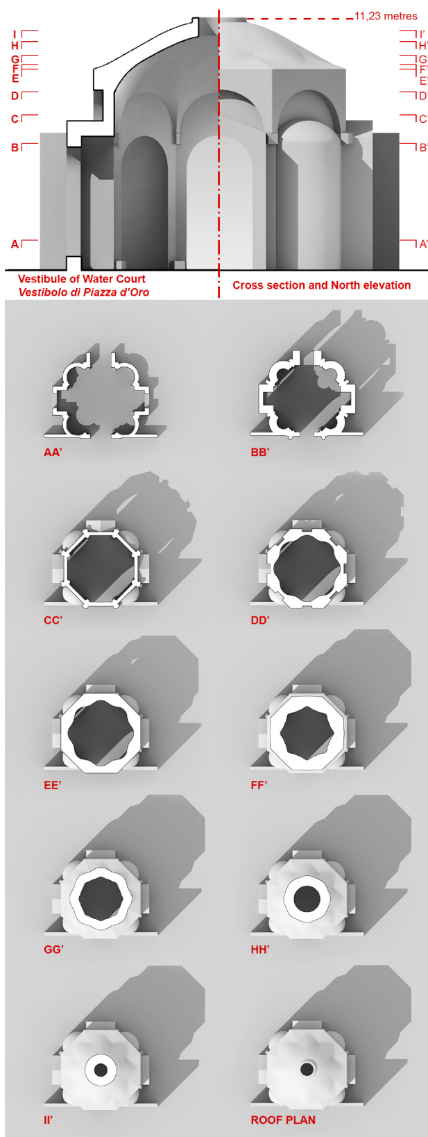
Figure 3. Vestibule of the Water Court. Rendering images of subsequent horizontal sections of the 3D procedural model of the Vestibule.
