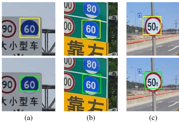
Fig. 11. Negative examples: (a) and (b) are caused by irregular target shapes. (c) target sign is bended, and it is no longer a planar shape.
