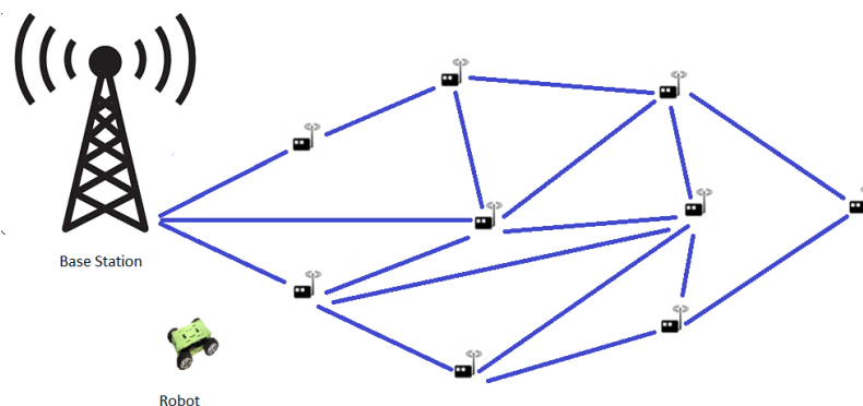
Figure 1. Sensor network for mobile robot charger.
