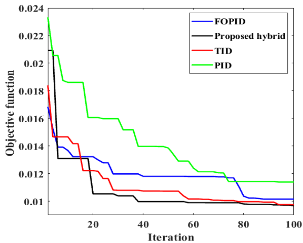
FIGURE 6: Convergence curve at scenario 1.
