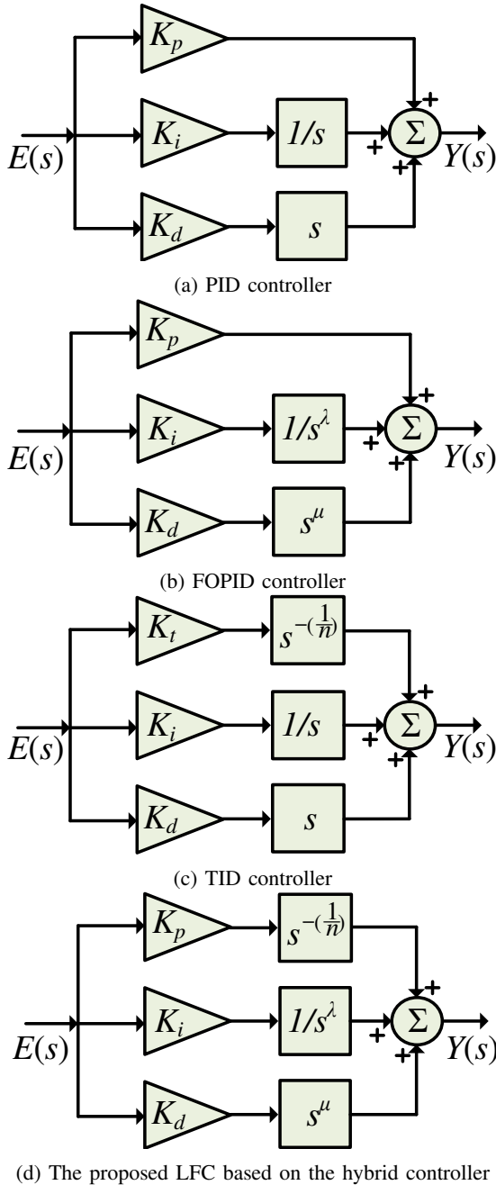
FIGURE 3: The block diagram of existing FO and the proposed LFC hybrid controller
