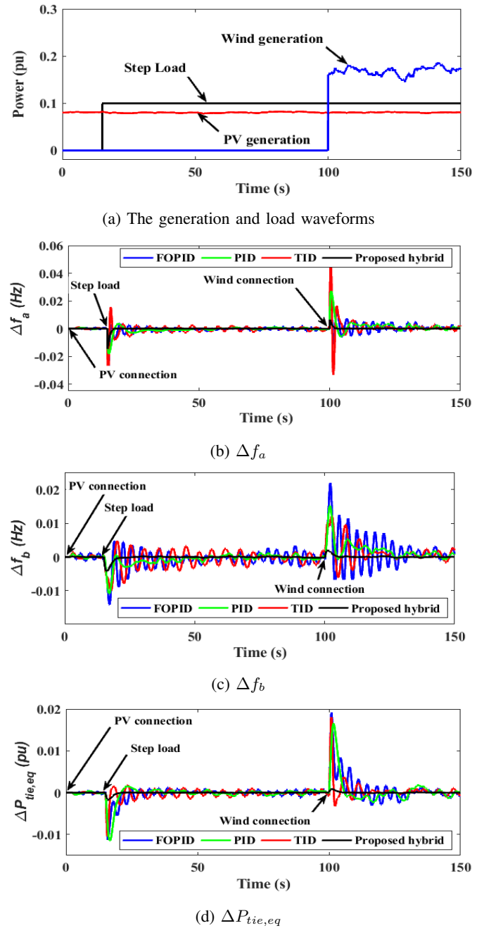
FIGURE 9: System response with the optimized controllers at scenario 2.
