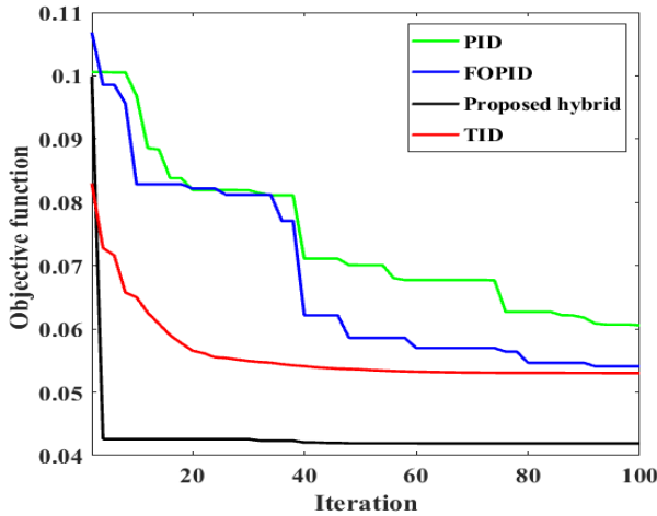
FIGURE 8: Convergence curve at scenario 2.
