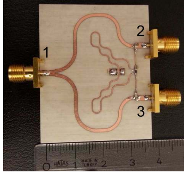
Fig. 14. Implemented 2-way power divider of Fig. 10.
