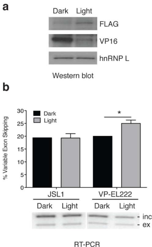
Figure 4. Light-regulated gene expression of the splicing factor CELF2 using VP-EL222 in the T-cell derived JSL1 cell line
