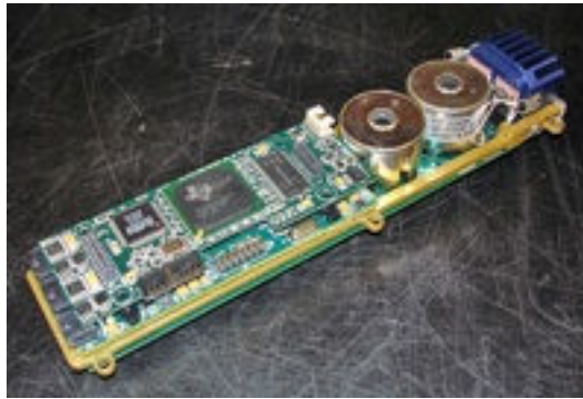
Figure 5: WHOI Acoustic Micro-Modem
