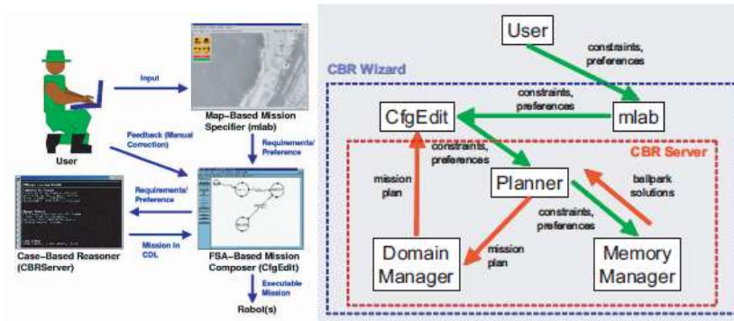
Figure 14: Overview of mission specification using the CBR Wizard. A user specifies the desired tasks using the map-based interface of MissionLab. CBRServer retrieves a mission based on the user’s input. The mission is presented for user inspection, modification, and execution.
