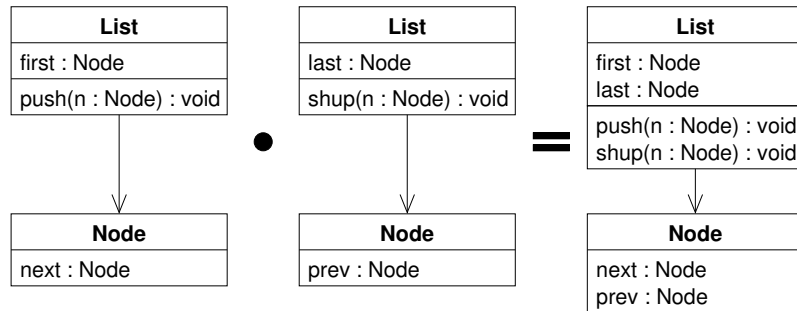
Figure 10: Feature composition involves model merging.
