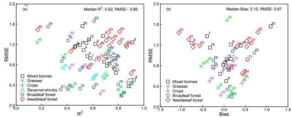
Figure 3. Statistical R-squared values ( R^2 ) and (a) root-mean-squared error (RMSE) and bias and (b) RMSE from direct validation of moderate resolution leaf area index products. The numbers correspond to the reference number in Table S2.
