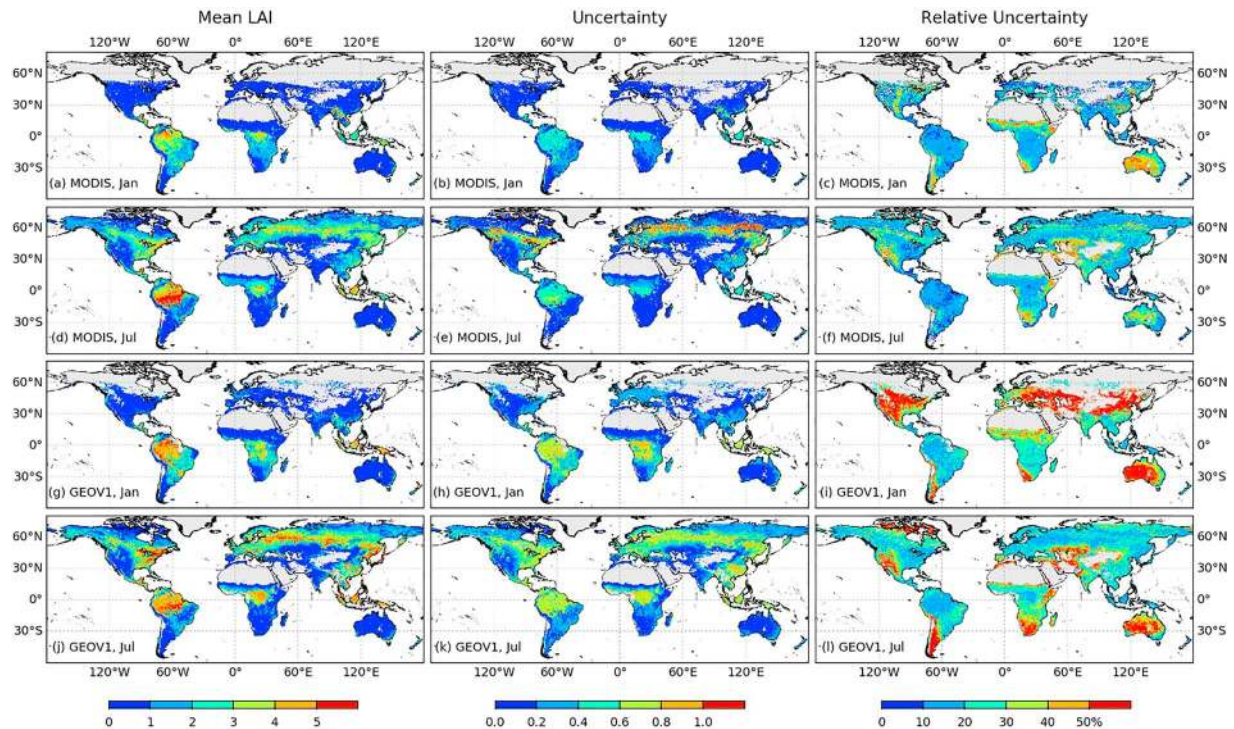
Figure 2. Global mean LAI (left), uncertainties (middle), and relative uncertainties (right) from MODIS (MOD15A2H, C6) and GEOV1 from 2003 to 2013 ( 0.05^\circ ) in January and July, respectively. The MODIS and GEOV1 uncertainties are derived from the standard deviation (LaiStdDev) and error (LAI_ERR) layers, respectively. The relative uncertainties are derived as a ratio of uncertainties to the mean LAI. LAI = leaf area index; MODIS = Moderate Resolution Imaging Spectroradiometer; GEOV1 = Geoland2/BiopPar version 1.
