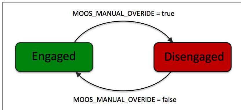
Figure 10: The Engagement state of the IvP Helm: The helm is either engaged or disengaged, depending on both how the helm is initialized and mail received by the helm after start-up on the variable MOOS_MANUAL_OVERRIDE . The value for this variable is case insensitive.
