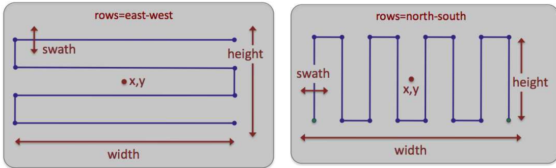
Figure 22: SegLists built with the lawnmower format: The pattern is specified by (a) the location of the center of the pattern, (b) the height and width of the pattern, (c) the lane width which determines the number of rows, (d) whether the pattern rows proceed north-south or east-west, and (e) an optional rotation of the pattern.
