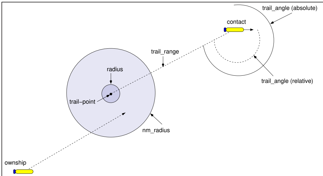
Figure 52: Interpolation of vehicle speed inside the radius set by NM_RADIUS relative to the extrapolated trail position.
