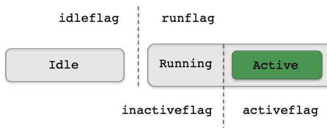
Figure 15: Behavior Flags: The four behavior flags idleflag , runflag , activeflag , and inactiveflag are posted depending on the behavior state and can be considered complementary in the manner indicated.
