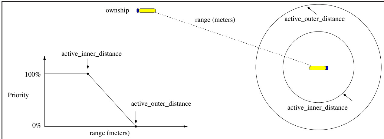
Figure 49: Parameters for the BHV_AvoidCollision behavior: The ownship vehicle is the platform running the helm. The range between the two vehicles affects whether the behavior is active and with what priority weight. Beyond the active_outer_distance , the behavior is not active. Within the active_inner_distance , the behavior is active with 100% of its priority weight.
