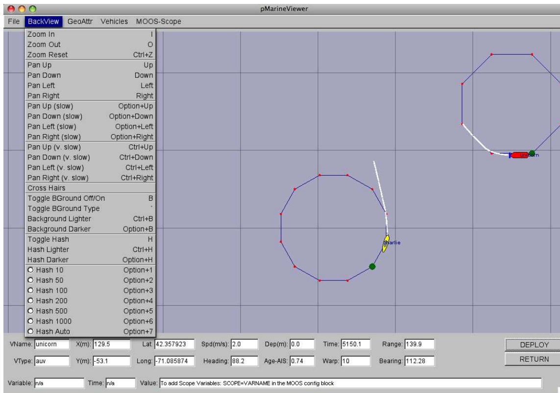
Figure 25: The BackView menu: This pull-down menu lists the options, with hot-keys, for affecting rendering aspects of the geo-display background.
