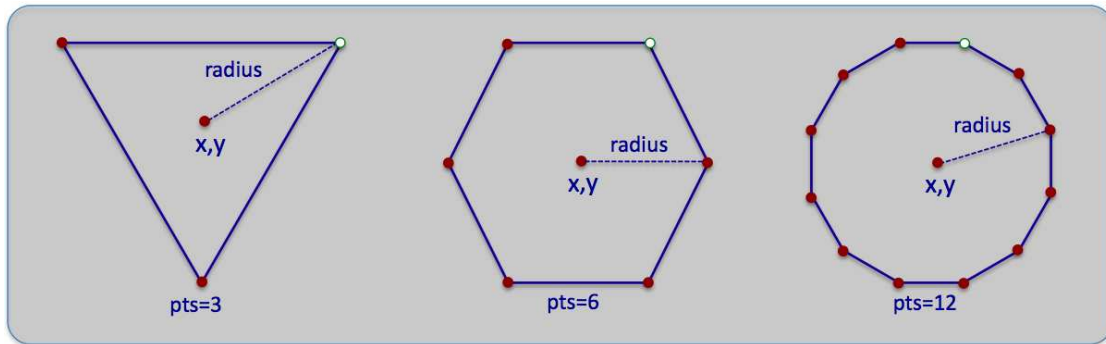
Figure 20: Polygons built with the radial format: Radial polygons are specified by (a) the location of their center, (b) the number of vertices, and (c) the radial distance from the center to each vertex. The lighter vertex in each polygon indicates the first vertex if traversing in sequence, proceeding clockwise.
