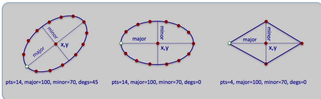
Figure 21: Polygons built with the ellipse format: Ellipse polygons are specified by (a) the location of their center, (b) the number of vertices, (c) the length of their major axis, (d) the length of their minor axis, and (e) the rotation of the ellipse. The lighter vertex in each polygon indicates the first vertex if traversing in sequence, proceeding clockwise.
