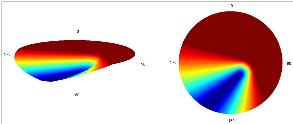
Figure 51: The objective function produced by the collision avoidance behavior is defined over possible heading and speed values. Higher speeds are represented farther radially out from the center.
