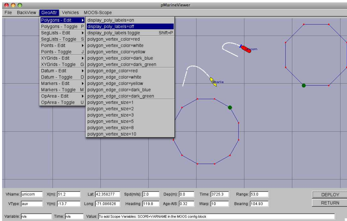
Figure 26: The GeoAttributes menu: This pull-down menu lists the options and hot keys for affecting the rendering of geometric objects.
