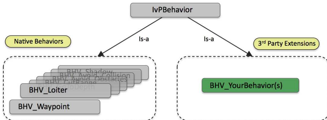
Figure 18: Behavior inheritance: Behaviors are derived from the IvPBehavior superclass. The native behaviors are the behaviors distributed with the helm. New behaviors also need to be subclass of the IvPBehavior class to work with the helm. Certain virtual functions invoked by the helm may be optionally but typically overloaded in all new behaviors. Other private functions may be invoked within a behavior function as a way of facilitating common tasks involved in implementing a behavior.
