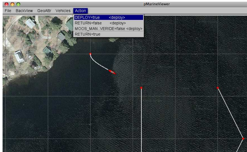
Figure 28: The Action menu: The variable value pairs on each menu item may be selected for poking or writing the MOOSDB. The three variable-value pairs above the menu divider will be poked in unison when any of the three are chosen, because they were configured with the same key, <deploy> , shown to the right on each item.
