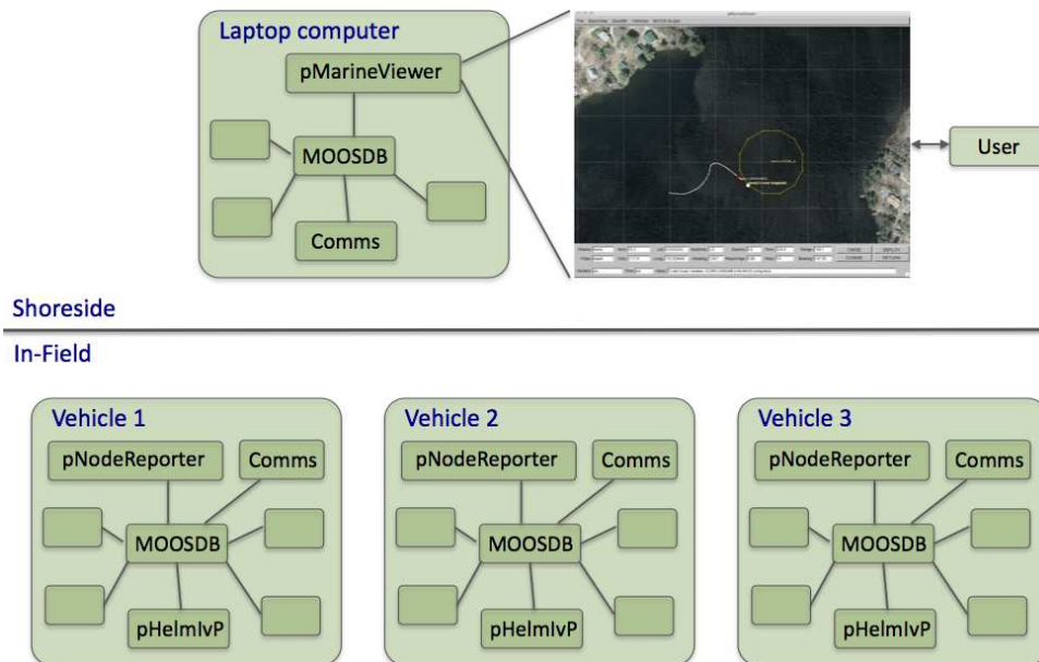
Figure 23: A common usage of the pMarineViewer is to have it running in a local MOOSDB community while receiving node reports on vehicle poise from other MOOS communities running on either real or simulated vehicles. The vehicles can also send messages with certain geometric information such as polygons and points that the view will accept and render.
