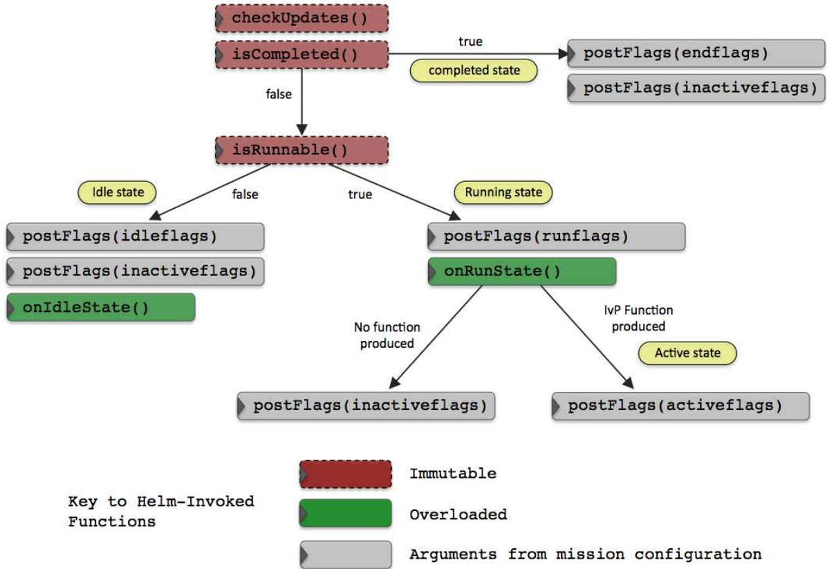
Figure 19: Behavior function-calls by the helm: The helm invokes a sequence of functions on each behavior on each iteration of the helm. The sequence of calls is dependent on what the behavior returns, and reflects the behaviors activity state. Certain functions are immutable and can not be overloaded by a behavior author. Two key functions, onRunState() and onIdleState() can be indeed overloaded as the usual hook for an author to provide the implementation of a behavior. The postFlags function is also immutable, but the parameters (flags) are provided in the helm configuration ( *.bhv ) file.
