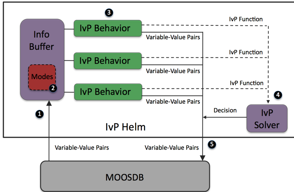
Figure 11: The pHelmIvP Iterate Loop : (1) Mail is read from the MOOSDB . It is parsed and stored in a local buffer to be available to the behaviors, (2) If there were any mode declarations in the mission behavior file they are evaluated at this step. (3) Each behavior is queried for its contribution and may produce an IvP function and a list of variable-value pairs to be posted to the MOOSDB at the end of the iteration, (4) the objective functions are resolved to produce an action, expressible as a set of variable-value pairs, (5) all variable-value pairs are published to the MOOSDB for other MOOS processes to consume.
