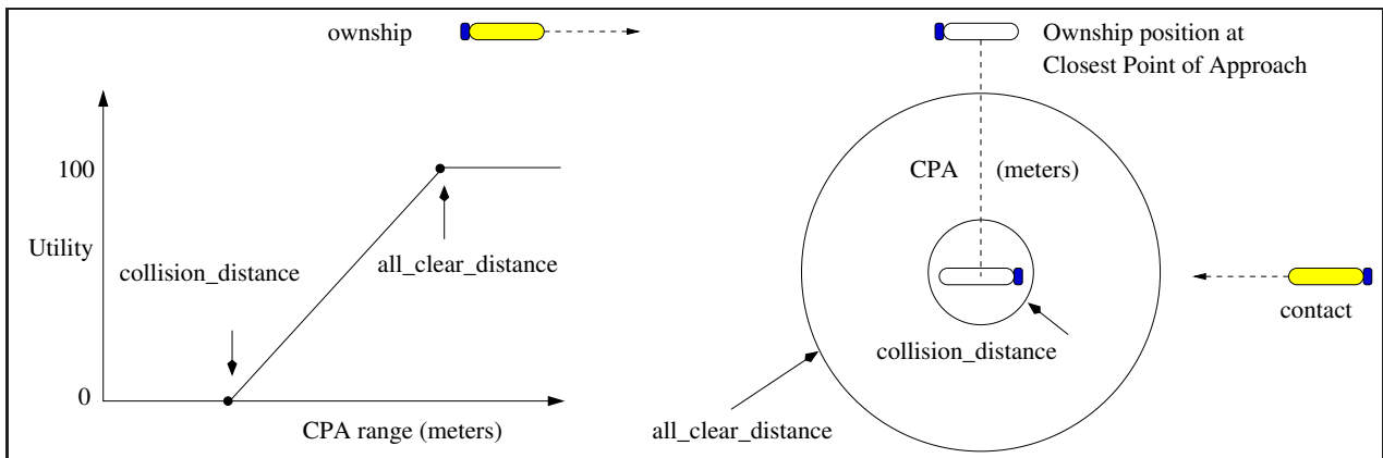
Figure 50: Parameters for the BHV_AvoidCollision behavior. The ownship vehicle is the platform running the helm. The collision_distance is used when applying a utility metric to a calculated closest point of approach (CPA) for a candidate maneuver. A CPA less than or equal to the collision_distance is treated as an actual collision with the lowest utility rating.
