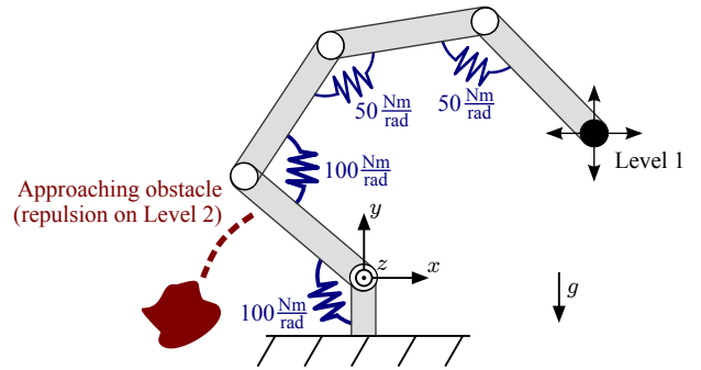
Figure 3: Simulation model of a planar, four DOF system. The links are connected via revolute joints. Each link is modeled by a point mass of 1 kg that is placed in the middle of a bar with length 0.5 m. The dynamics are simulated using g = 9.81 \text{ m/s}^2 . As depicted, four mechanical springs are placed in between the links. These allow to maintain a TCP position without active control and power consumption. Additional joint damping is introduced with d_i = 15 \text{ Nms/rad} for i = 1, 2, 3, 4 so that no DOF are undamped.
