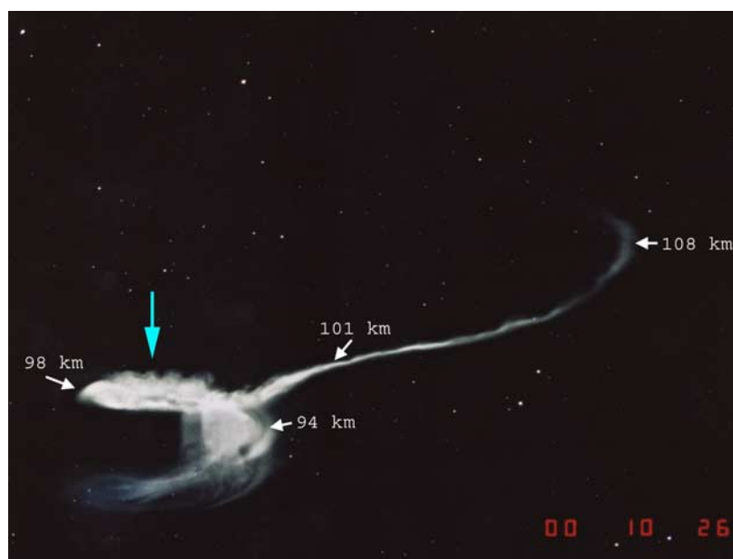
Figure 5. A photograph of the TMA trail on the downleg. The arrow points to the KH billows which occur between 96 and 99 km.
